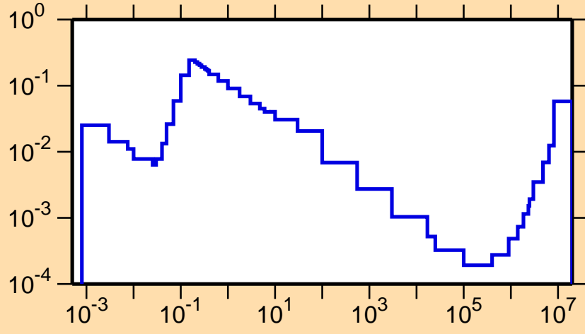
\sigma vs. E for ^{141}\text{Eu}(n,\alpha)
