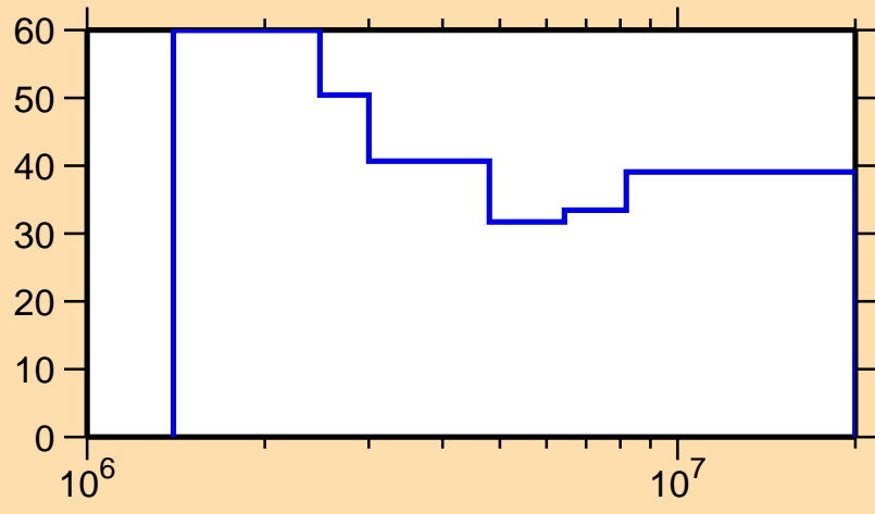
\Delta\sigma/\sigma vs. E for ^{141}\text{Eu}(n,n\text{cont.})
