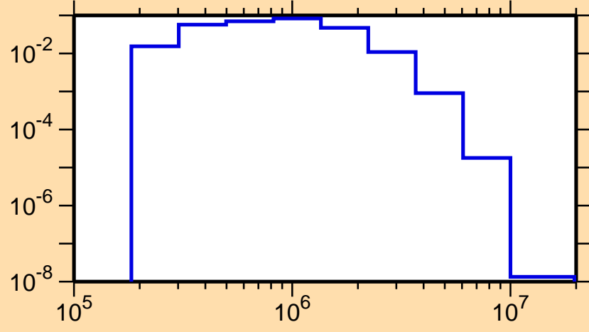
\sigma vs. E for ^{141}\text{Eu}(n,n_3)
