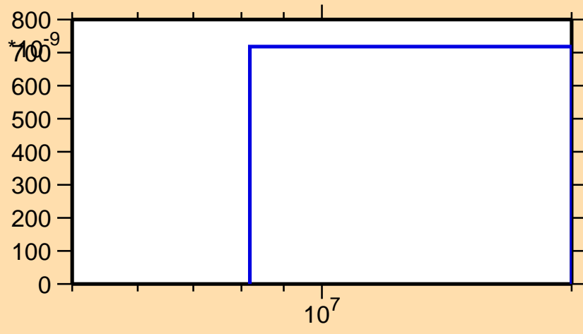
\sigma vs. E for ^{141}\text{Eu}(\text{mt } 45)
