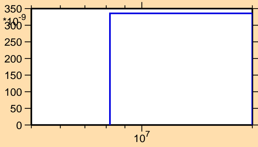
\sigma vs. E for ^{141}\text{Eu}(n,\text{pd})
