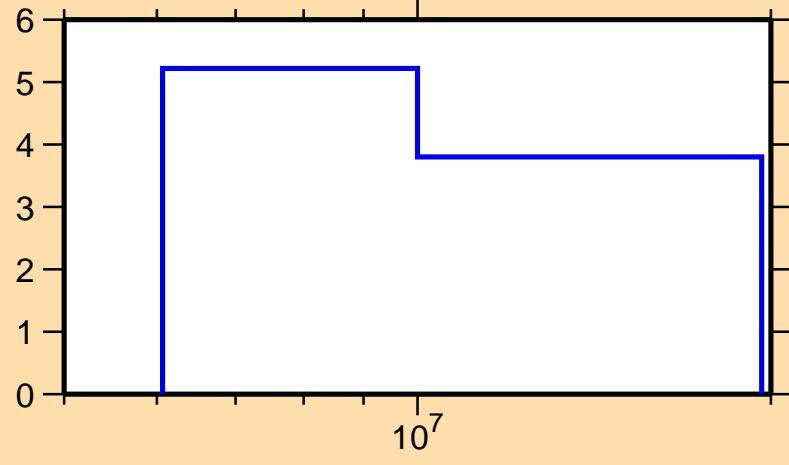
\Delta\sigma/\sigma vs. E for ^{142}\text{Eu}(n,\text{el.})
