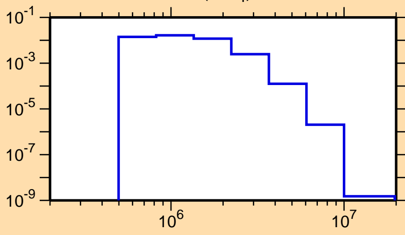
\sigma vs. E for ^{142}\text{Eu}(n,n_4)
