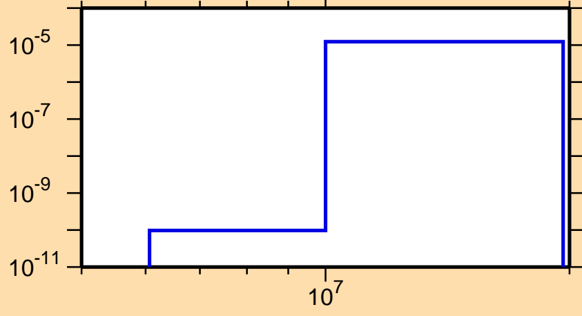
\sigma vs. E for ^{142}\text{Eu}(n,\text{He3})
