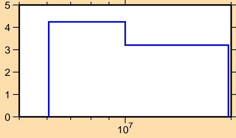
\Delta\sigma/\sigma vs. E for ^{142}\text{Eu}(n,\text{tot.})
