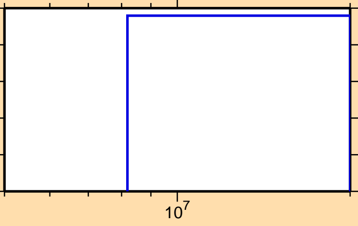
\sigma vs. E for ^{142}\text{Eu}(n,2np)
