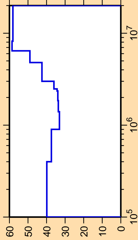
\Delta\sigma/\sigma vs. E for ^{142}\text{Eu}(n,n_2)
