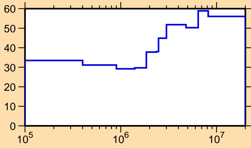
\Delta\sigma/\sigma vs. E for ^{142}\text{Eu}(n,n_1)
