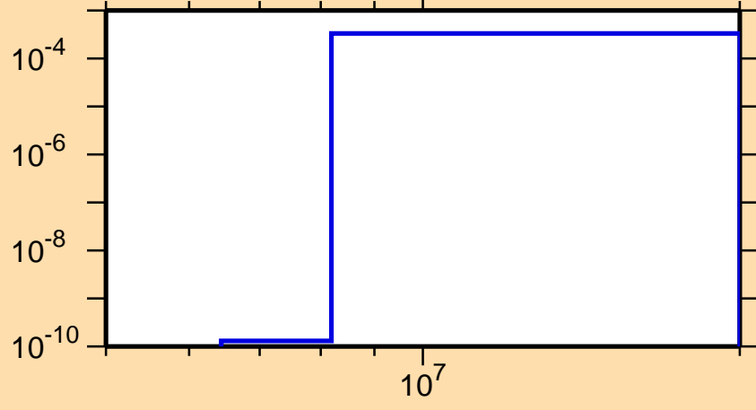
\sigma vs. E for ^{142}\text{Eu}(n,t)
