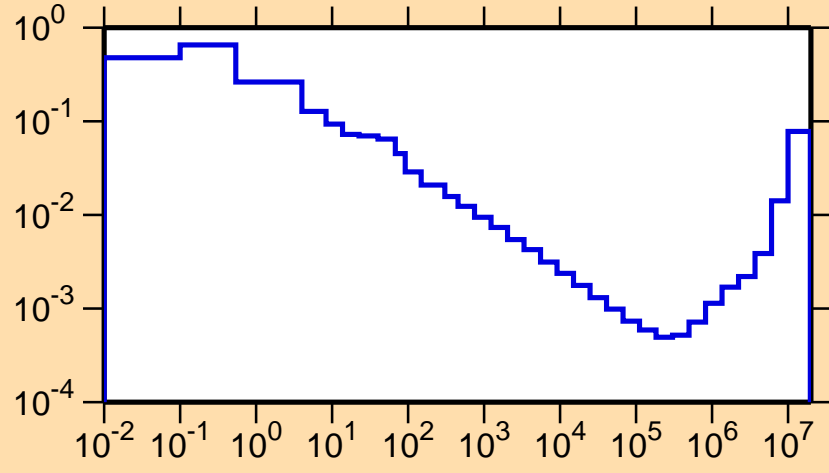
\sigma vs. E for ^{142}\text{Eu}(n,\alpha)
