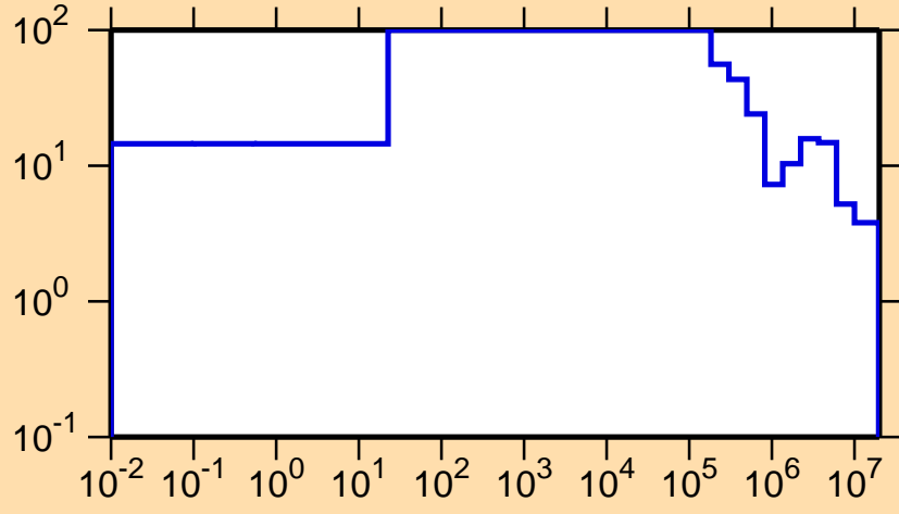
\Delta\sigma/\sigma vs. E for ^{142}\text{Eu}(n, el.)
