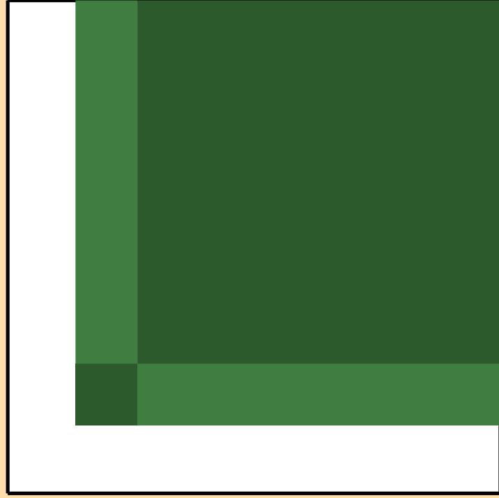
\sigma vs. E for ^{143}\text{Eu}(n,2n)
