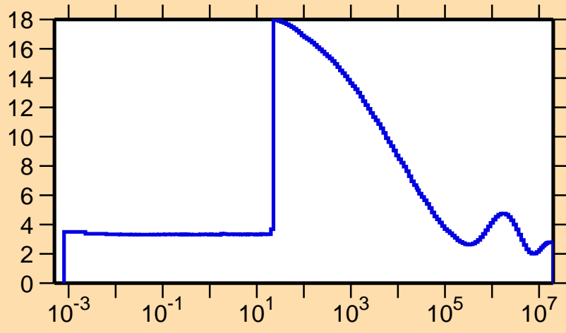
\sigma vs. E for ^{143}\text{Eu}(n,\text{el.})
