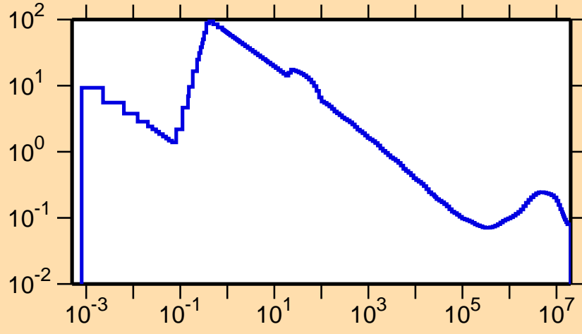
\sigma vs. E for ^{143}\text{Eu}(n,p)
