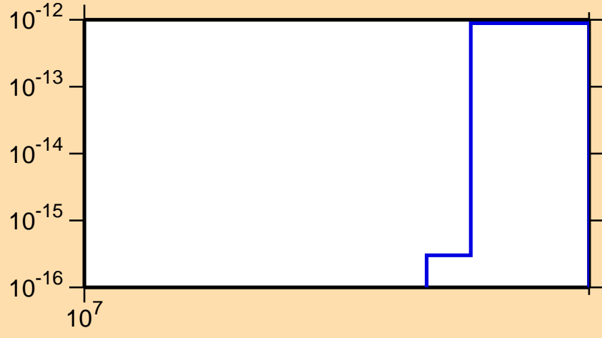
\sigma vs. E for ^{143}\text{Eu} (mt 34)
