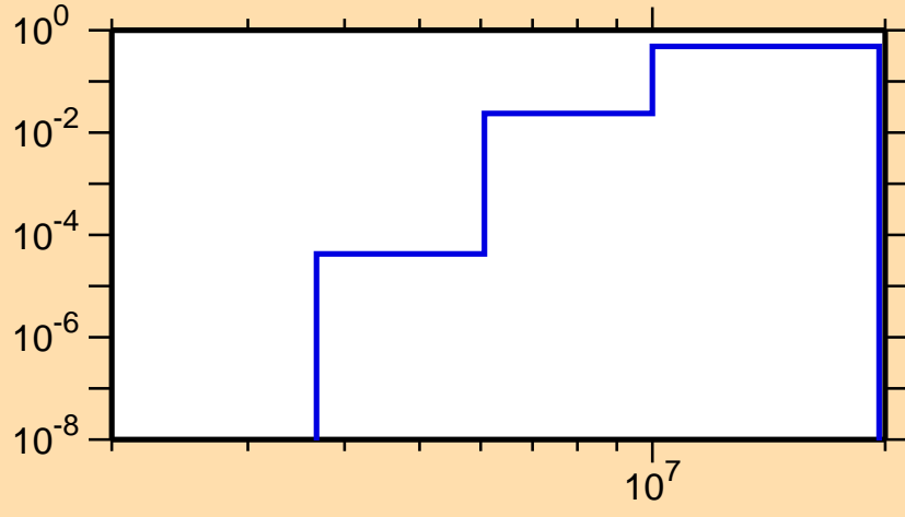
\sigma vs. E for ^{143}\text{Eu}(n,np)
