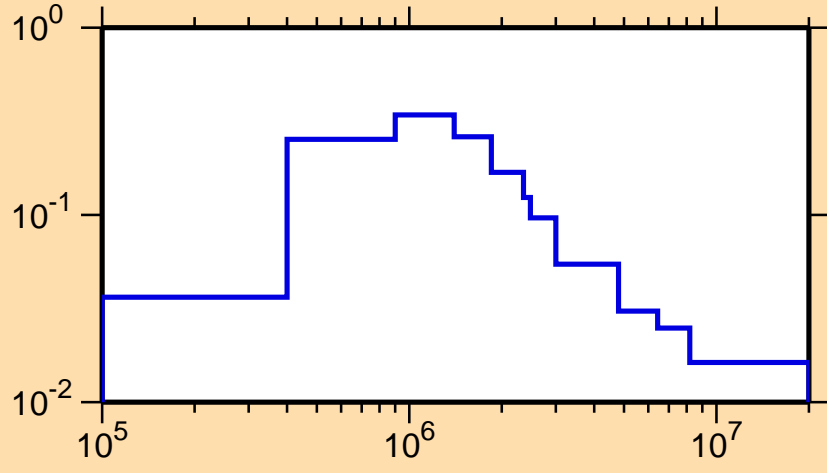
\sigma vs. E for ^{143}\text{Eu}(n,n_2)
