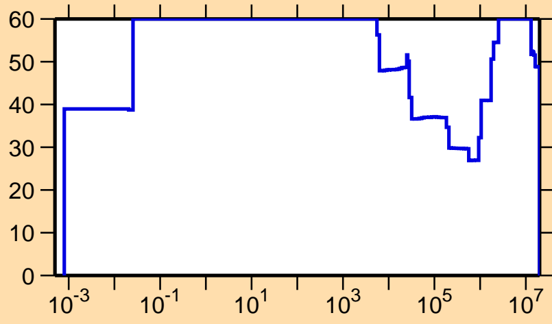
\Delta\sigma/\sigma vs. E for ^{144}\text{Eu}(n,p)
