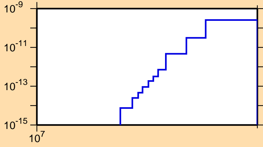
\sigma vs. E for ^{144}\text{Eu}(\text{mt117})
