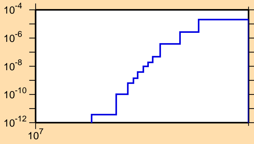
\sigma vs. E for ^{144}\text{Eu}(n,nd)
