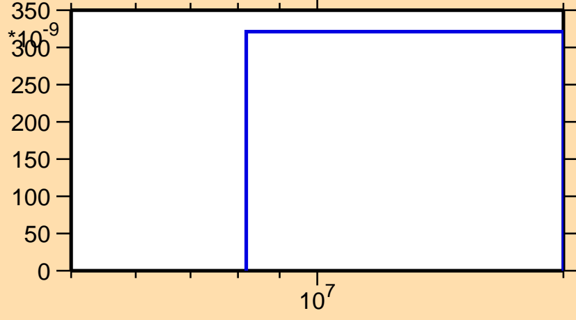
\sigma vs. E for ^{144}\text{Eu}(n,nd)
