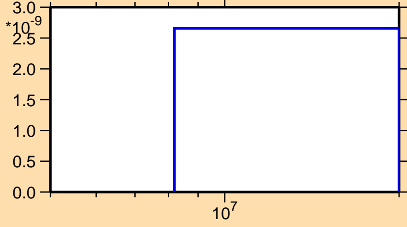
\sigma vs. E for ^{144}\text{Eu}(n,pd)
