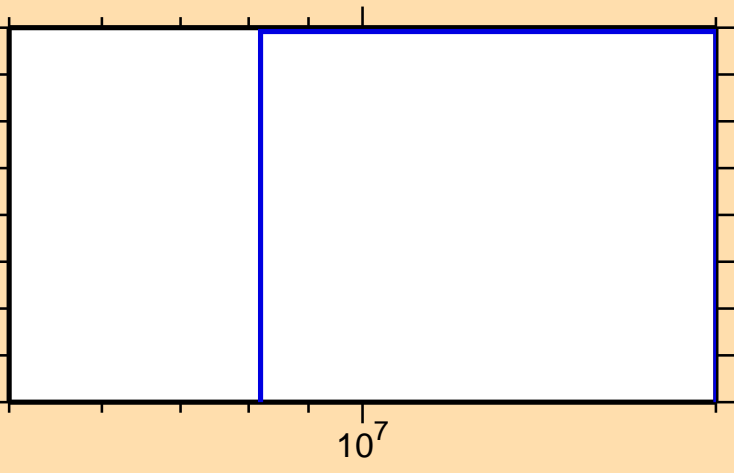
\sigma vs. E for ^{144}\text{Eu}(\text{mt117})
