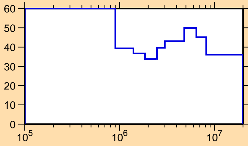
\Delta\sigma/\sigma vs. E for ^{144}\text{Eu}(n,n_1)
