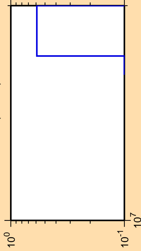
\Delta\sigma/\sigma vs. E for ^{145}\text{Eu} (mt 34)
