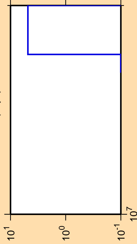
\Delta\sigma/\sigma vs. E for ^{145}\text{Eu}(n,\text{pt})
