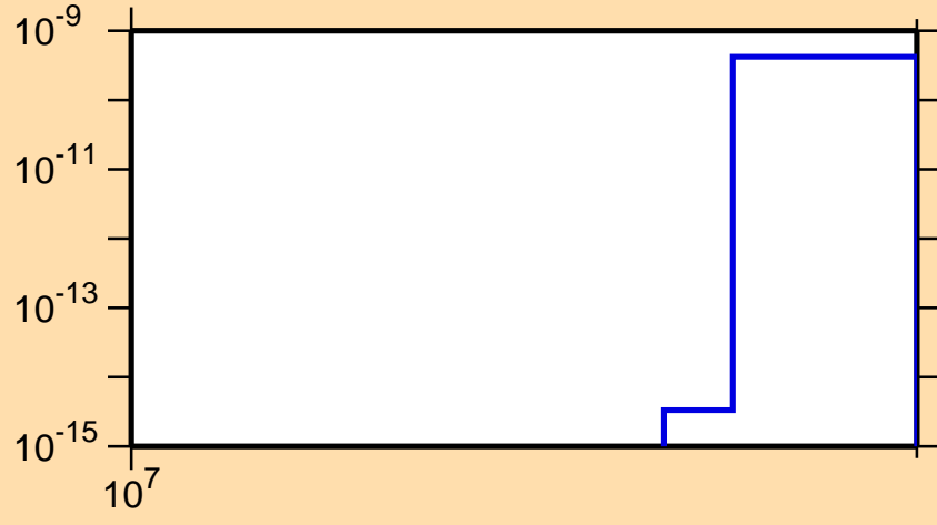
\sigma vs. E for ^{145}\text{Eu}(n,nt)
