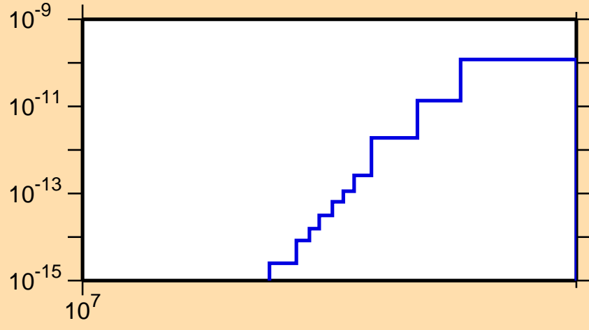
\sigma vs. E for ^{145}\text{Eu}(\text{mt117})
