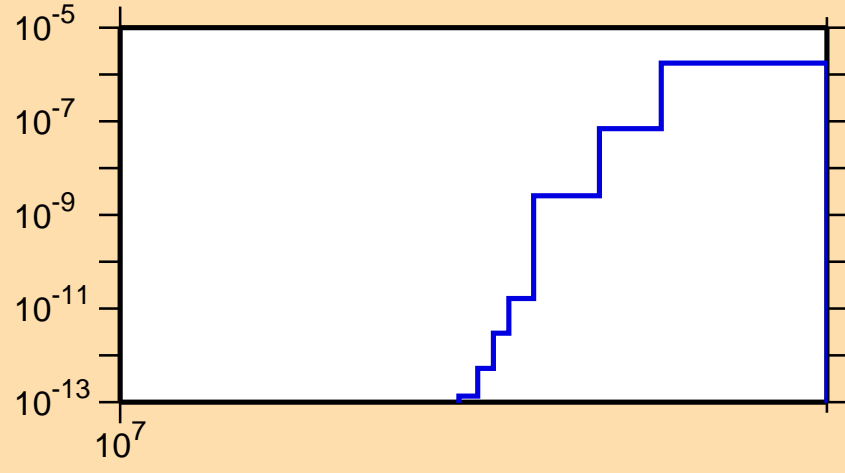
\sigma vs. E for ^{145}\text{Eu}(n,nd)
