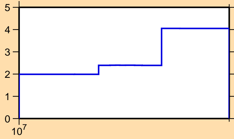
\Delta\sigma/\sigma vs. E for ^{145}\text{Eu}(n,\text{tot.})
