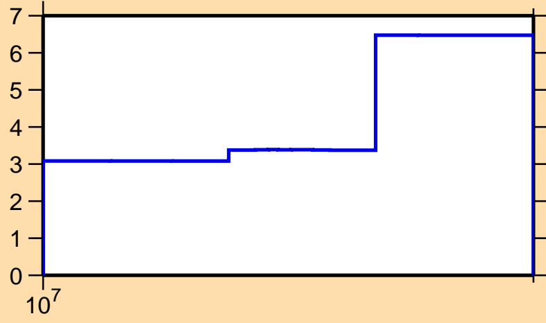
\Delta\sigma/\sigma vs. E for ^{145}\text{Eu}(n,\text{el.})
