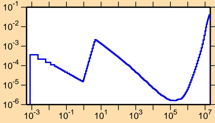
\sigma vs. E for ^{145}\text{Eu}(n,\alpha)
