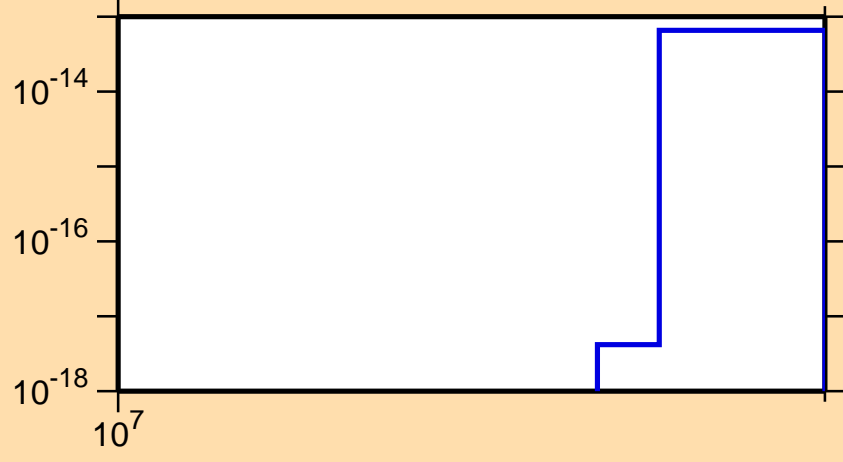
\sigma vs. E for ^{145}\text{Eu} (mt 34)
