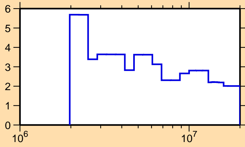
\Delta\sigma/\sigma vs. E for ^{145}\text{Eu}(n,\text{nonel.})
