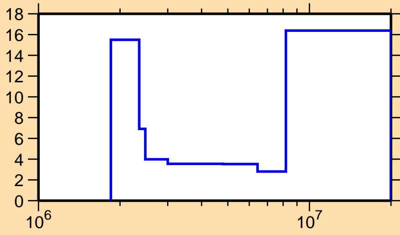
\Delta\sigma/\sigma vs. E for ^{145}\text{Eu}(n,n\text{cont.})
