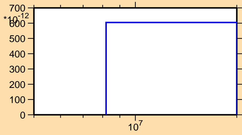
\sigma vs. E for ^{145}\text{Eu}(n,\text{pd})
