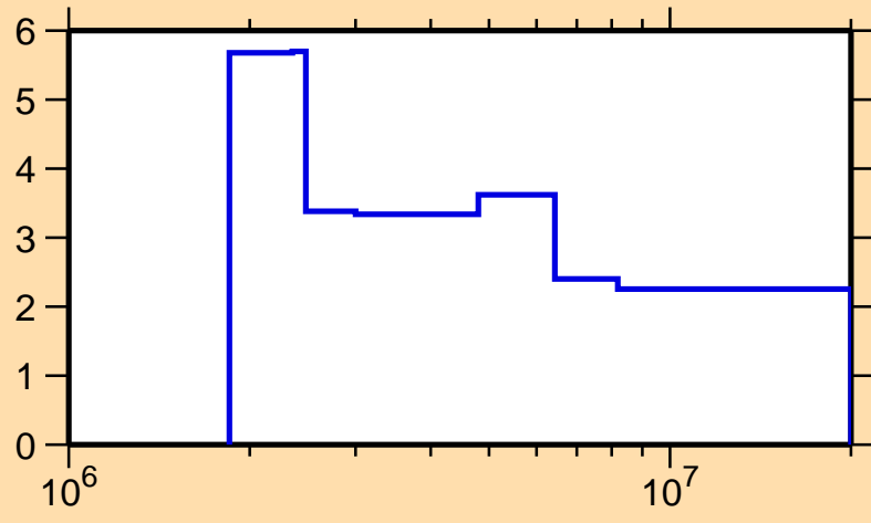
\Delta\sigma/\sigma vs. E for ^{145}\text{Eu}(n, n_{\text{nonel}})
