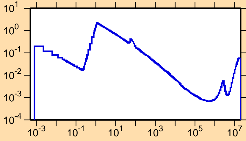
\sigma vs. E for ^{146}\text{Eu}(n,\alpha)
