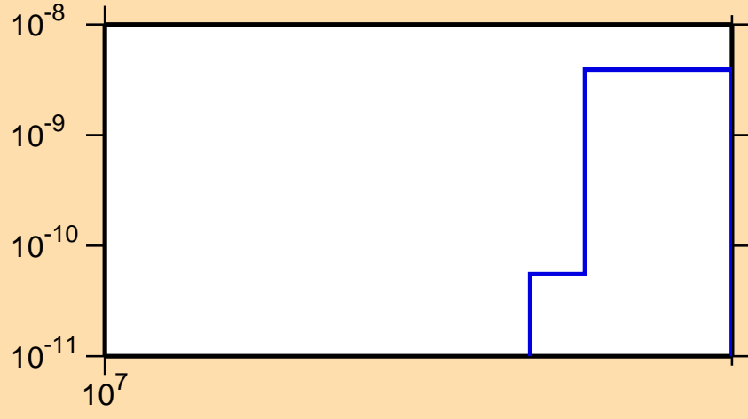
\sigma vs. E for ^{146}\text{Eu}(n,pt)
