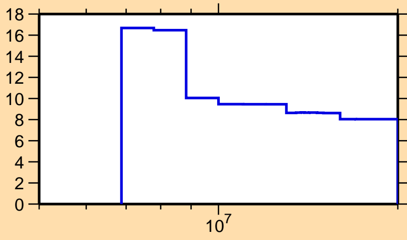
\Delta\sigma/\sigma vs. E for ^{146}\text{Eu}(n,2n)
