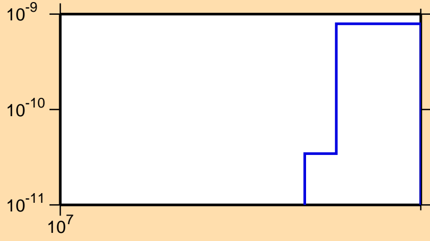
\sigma vs. E for ^{146}\text{Eu}(n,\text{pd})
