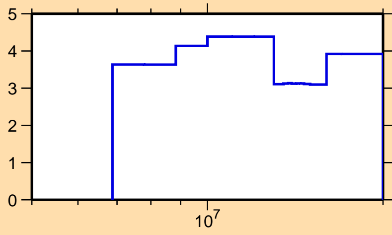
\Delta\sigma/\sigma vs. E for ^{146}\text{Eu}(n,\text{el.})
