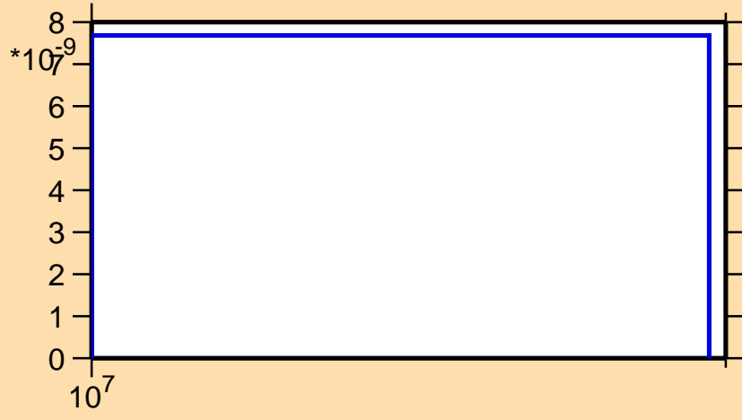
\sigma vs. E for ^{146}\text{Eu}(n,2n\alpha)
