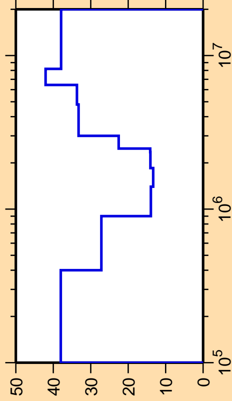
\Delta\sigma/\sigma vs. E for ^{146}\text{Eu}(n,n_4)
