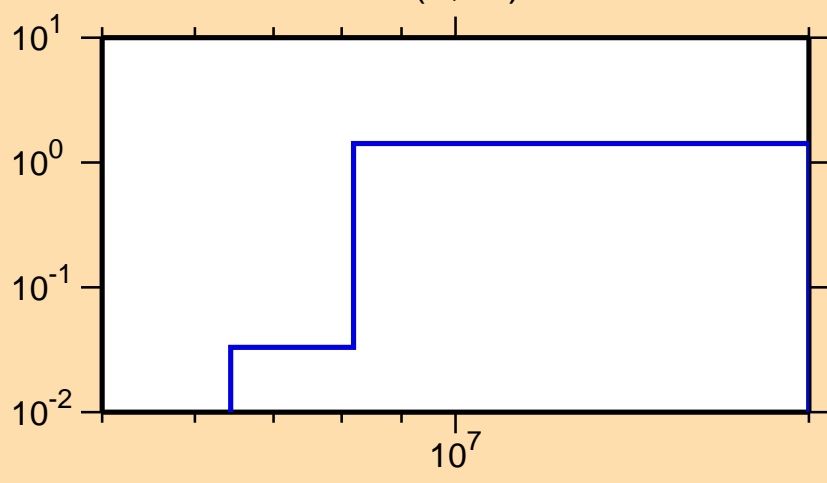
\sigma vs. E for ^{146}\text{Eu}(n,2n)
