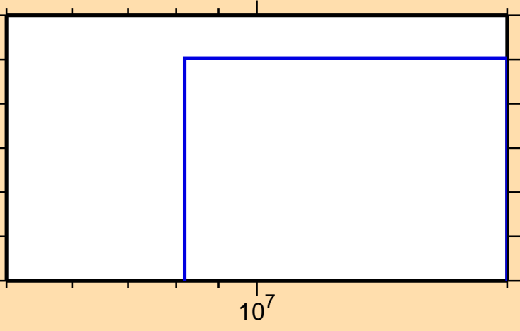
\sigma vs. E for ^{146}\text{Eu}(n,3n)
