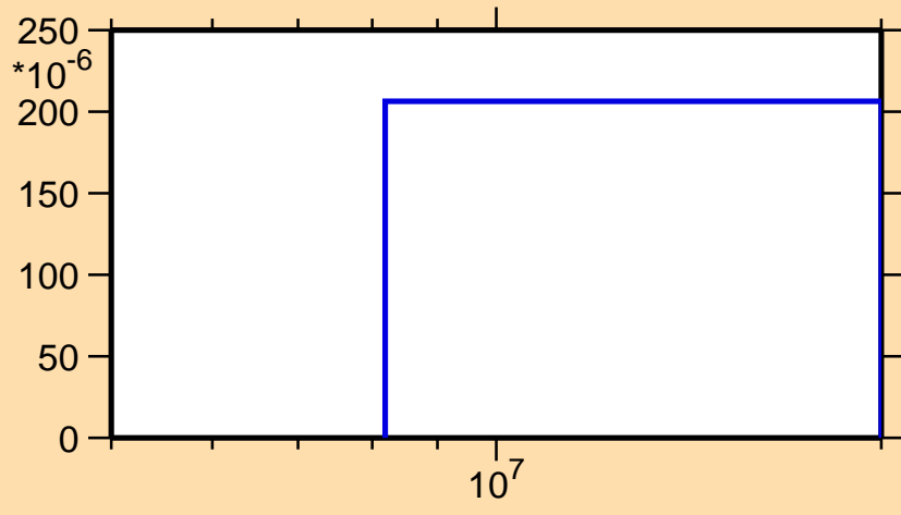
\sigma vs. E for ^{146}\text{Eu}(n,2np)
