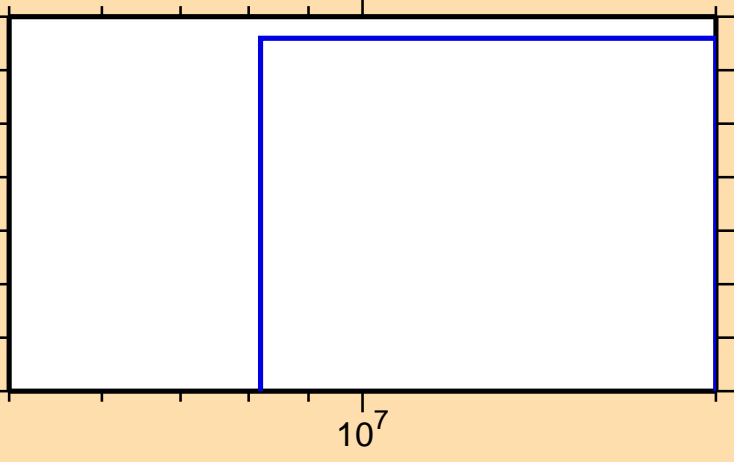
\sigma vs. E for ^{146}\text{Eu}(n,2n\alpha)
