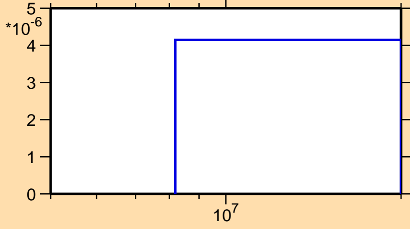
\sigma vs. E for ^{146}\text{Eu}(n,nd)
