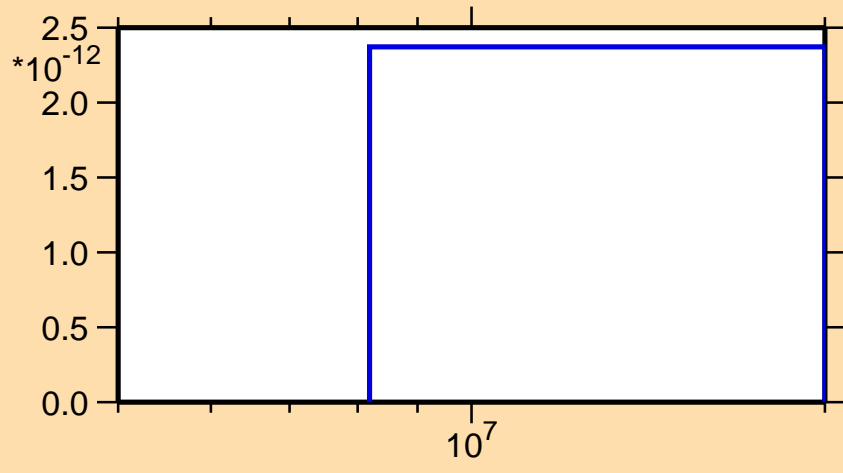
\sigma vs. E for ^{146}\text{Eu}(\text{mt } 34)
