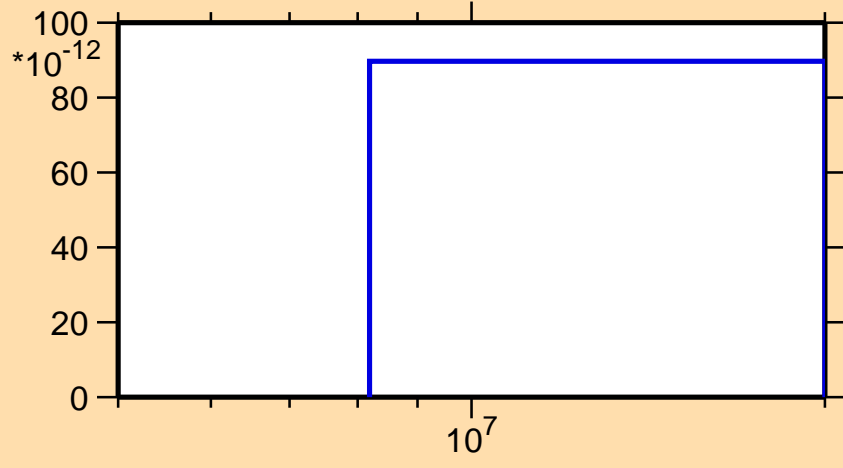
\sigma vs. E for ^{146}\text{Eu} (mt 45)
