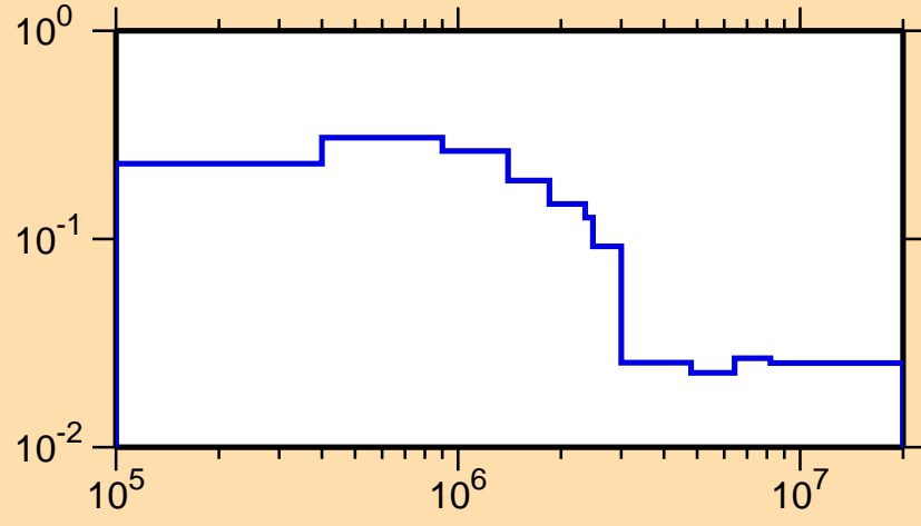
\sigma vs. E for ^{146}\text{Eu}(n,n_2)
