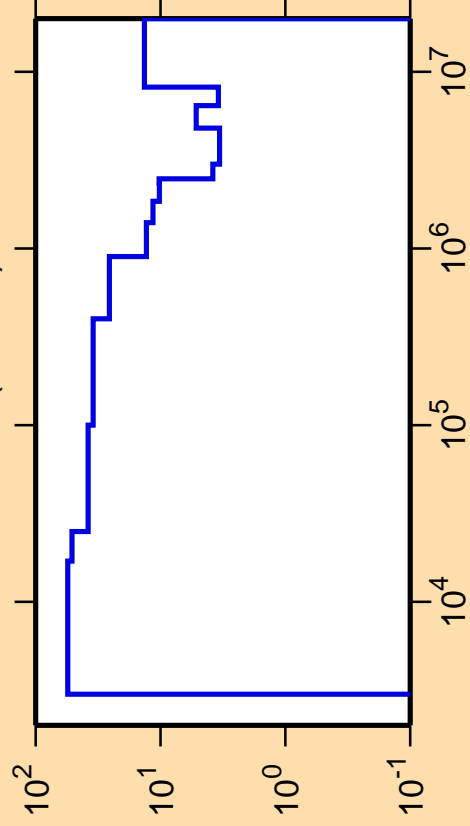
\Delta\sigma/\sigma vs. E for ^{146}\text{Eu}(n,\text{inel.})
