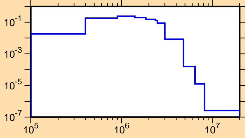
\sigma vs. E for ^{146}\text{Eu}(n,n_4)
