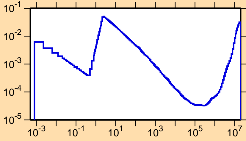
\sigma vs. E for ^{147}\text{Eu}(n,\alpha)
