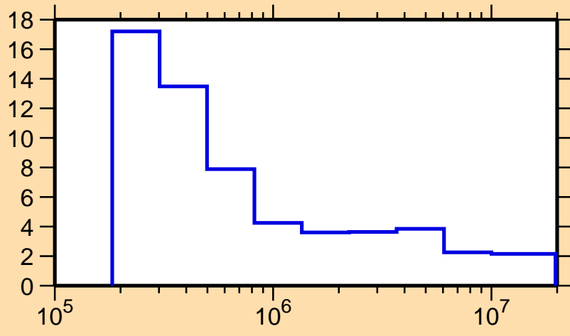
\Delta\sigma/\sigma vs. E for ^{147}\text{Eu}(n,\text{tot.})
