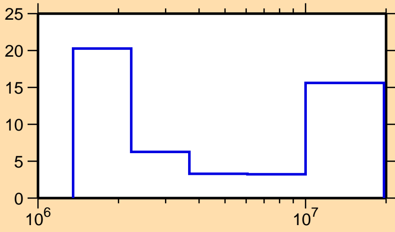
\Delta\sigma/\sigma vs. E for ^{147}\text{Eu}(n,n\text{cont.})
