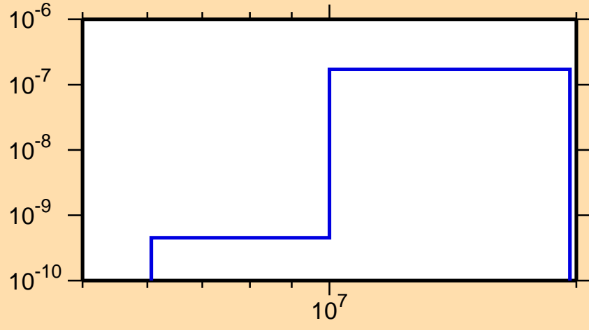
\sigma vs. E for ^{147}\text{Eu}(n,p\alpha)
