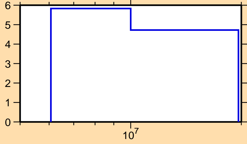
Delta \sigma/\sigma vs. E for ^{147}\text{Eu}(n,2n)
