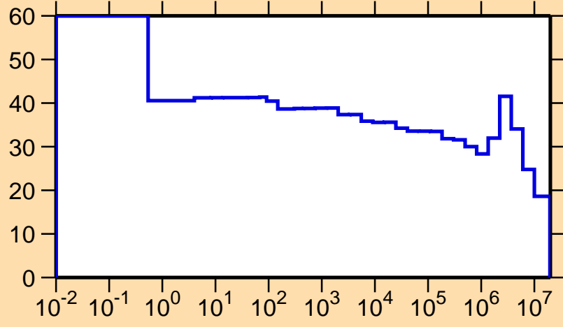
\Delta\sigma/\sigma vs. E for ^{147}\text{Eu}(n,p)
