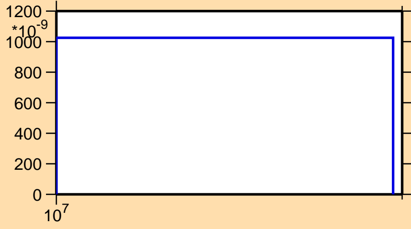
\sigma vs. E for ^{147}\text{Eu}(n,\text{nd})
