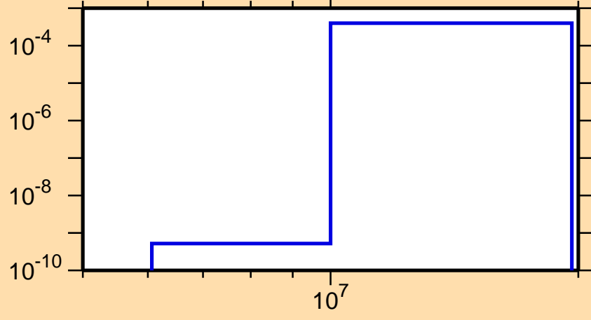
\sigma vs. E for ^{147}\text{Eu}(n,t)
