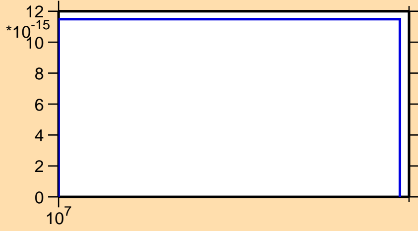
\sigma vs. E for ^{147}\text{Eu}(n,pt)
