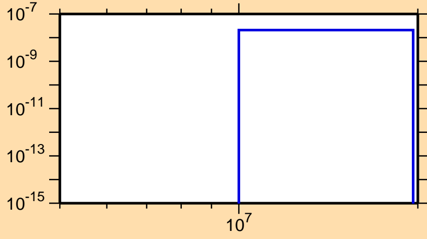
\sigma vs. E for ^{147}\text{Eu}(n,\text{He3})
