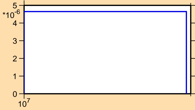
\sigma vs. E for ^{147}\text{Eu}(n,2np)
