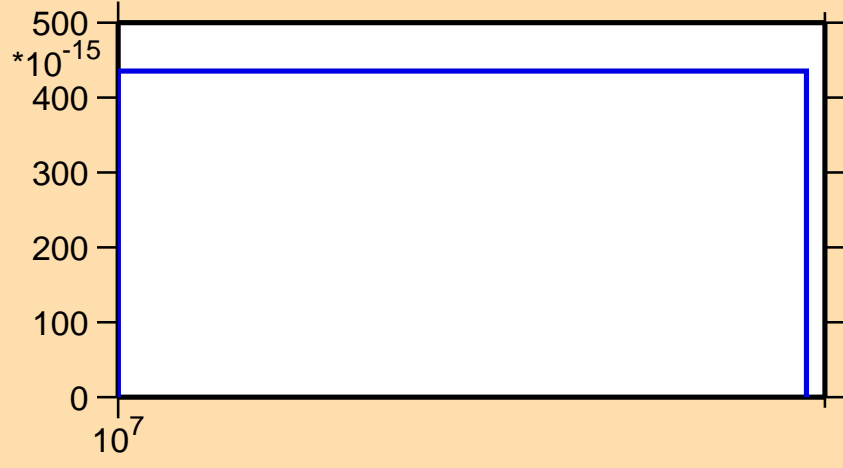
\sigma vs. E for ^{147}\text{Eu}(n,\text{pd})
