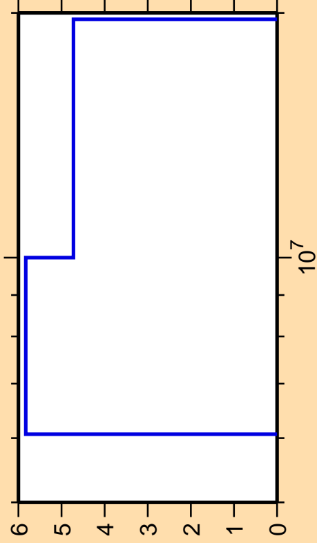
\Delta\sigma/\sigma vs. E for ^{147}\text{Eu}(n,2n)
