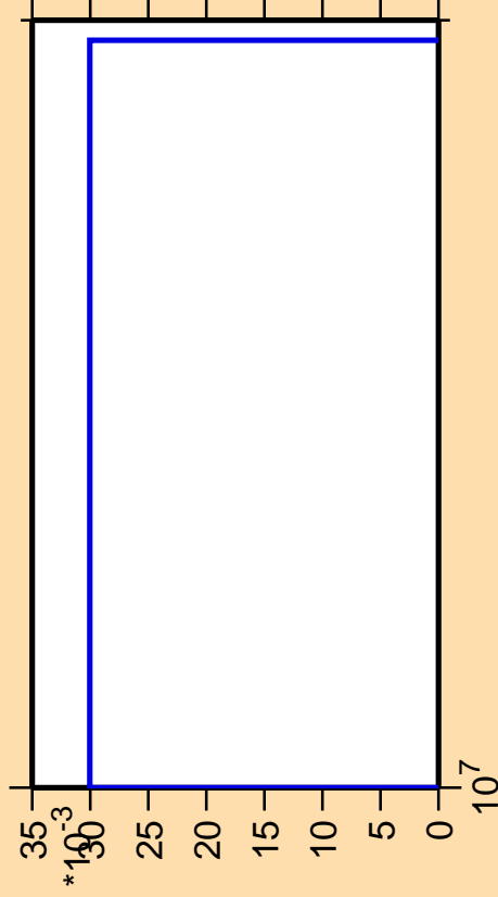
\Delta\sigma/\sigma vs. E for ^{147}\text{Eu}(n,pt)
