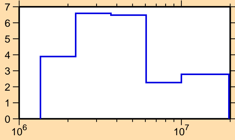
\Delta\sigma/\sigma vs. E for ^{147}\text{Eu}(n,\text{el.})
