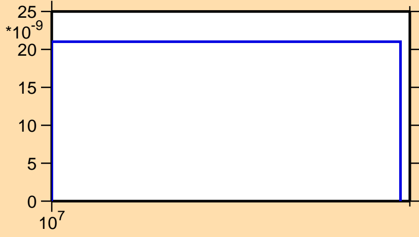
\sigma vs. E for ^{147}\text{Eu}(n,2n\alpha)
