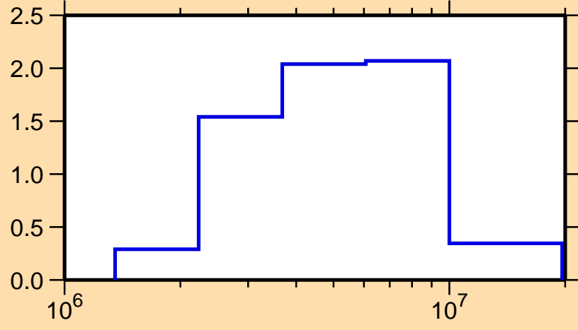
\sigma vs. E for ^{147}\text{Eu}(n,n\text{cont.})
