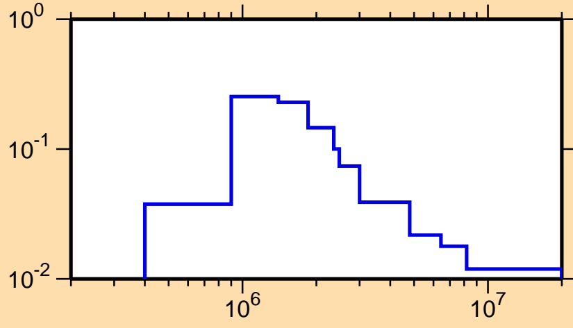
\sigma vs. E for ^{147}\text{Eu}(n,n_3)
