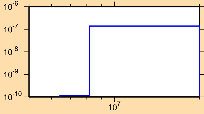
\sigma vs. E for ^{147}\text{Eu}(n,p\alpha)
