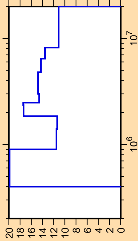
\Delta\sigma/\sigma vs. E for ^{147}\text{Eu}(n,n_3)
