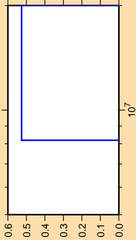
\Delta\sigma/\sigma vs. E for ^{147}\text{Eu}(n,pd)
