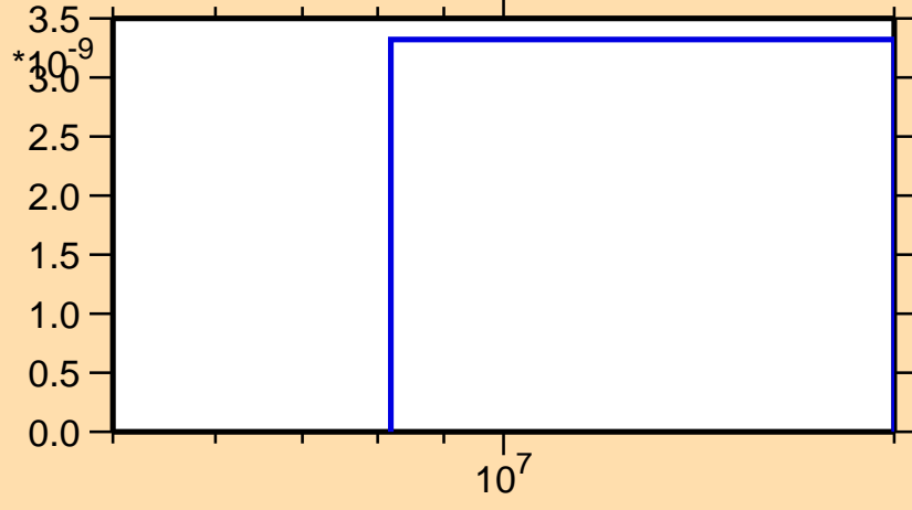
\sigma vs. E for ^{147}\text{Eu} (mt 45)
