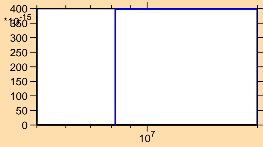
\sigma vs. E for ^{147}\text{Eu}(n,pd)
