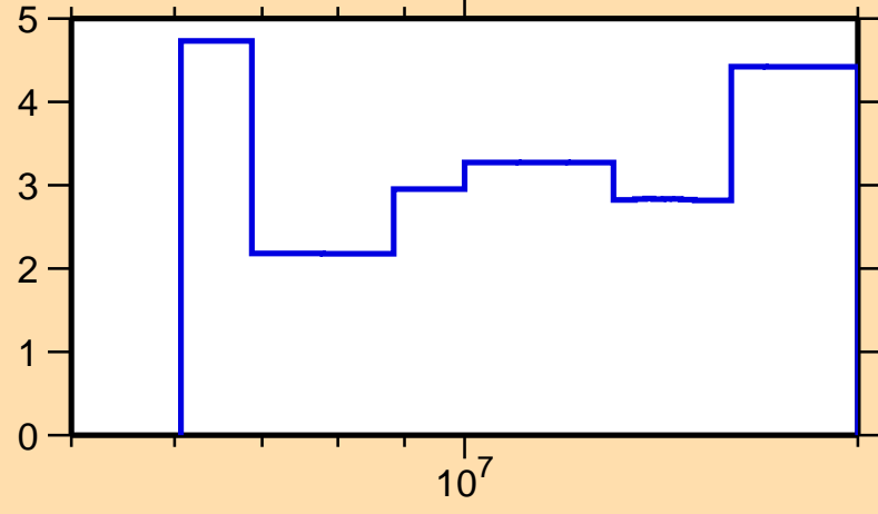
\Delta\sigma/\sigma vs. E for ^{148}\text{Eu}(n,\text{el.})
