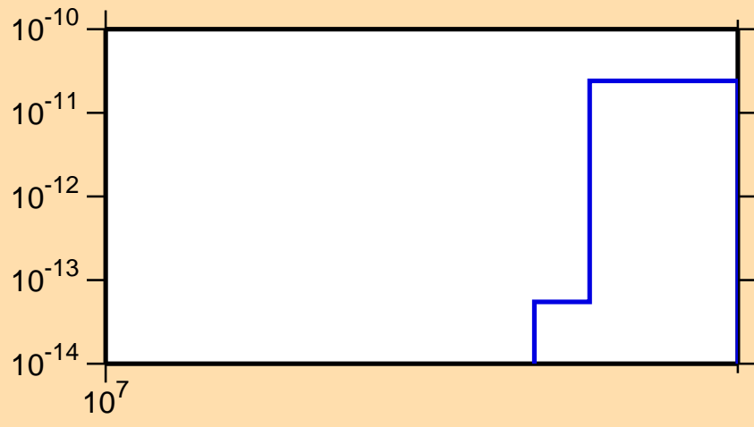
\sigma vs. E for ^{148}\text{Eu} (mt 34)
