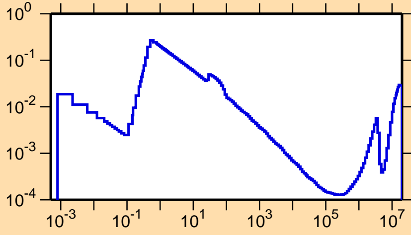
\sigma vs. E for ^{148}\text{Eu}(n,\alpha)
