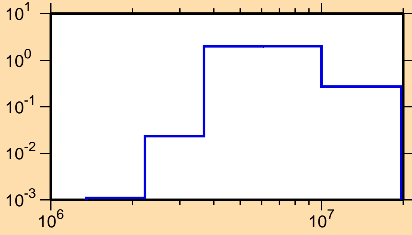
\sigma vs. E for ^{148}\text{Eu}(n,n\text{cont.})
