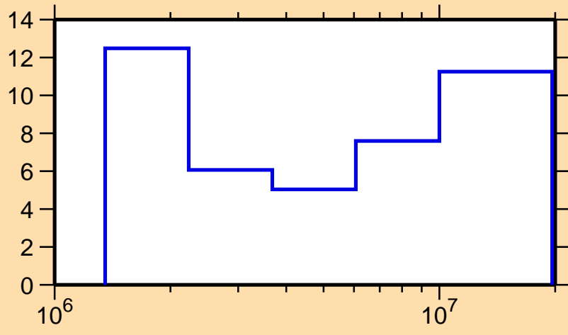
\Delta\sigma/\sigma vs. E for ^{148}\text{Eu}(n,n\text{cont.})
