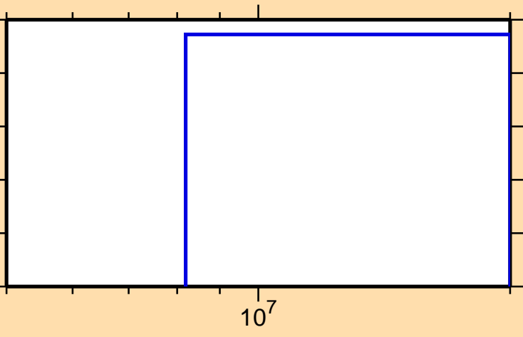
\sigma vs. E for ^{148}\text{Eu}(n,2np)
