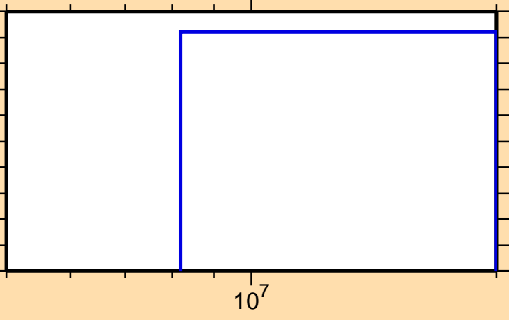
\sigma vs. E for ^{148}\text{Eu}(n,2n\alpha)
