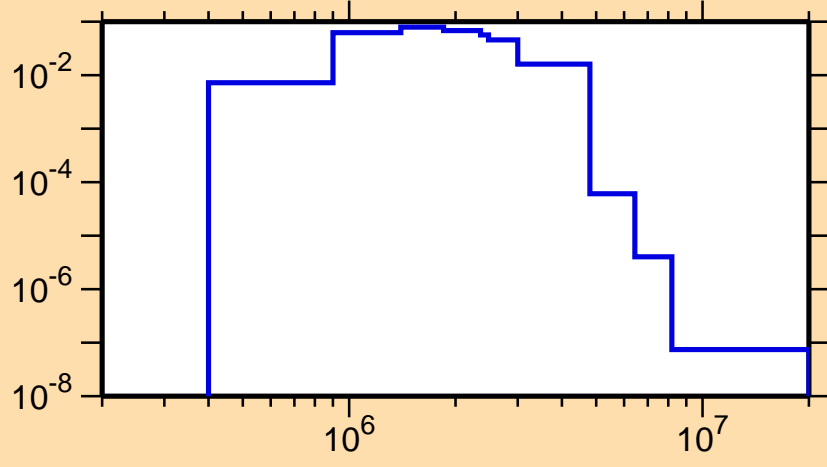
\sigma vs. E for ^{148}\text{Eu}(n,n_4)
