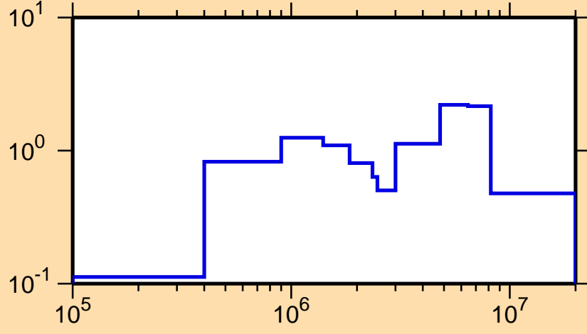
\sigma vs. E for ^{148}\text{Eu}(n,\text{inel.})
