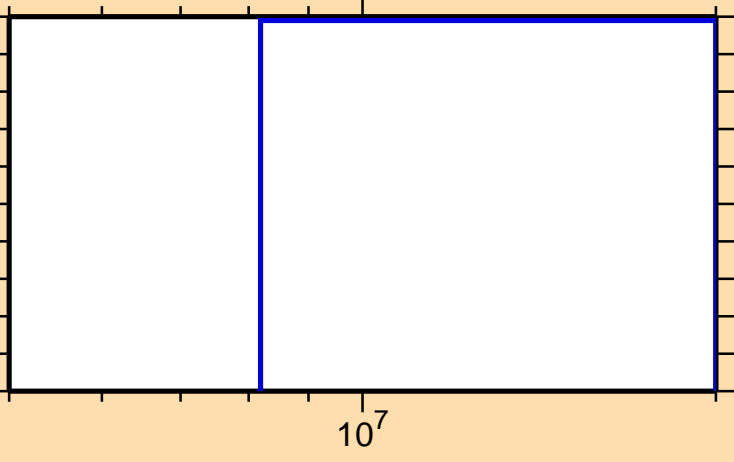
\sigma vs. E for ^{148}\text{Eu}(\text{mt } 34)
