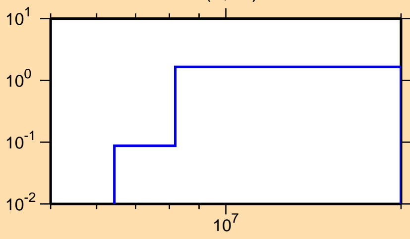
\sigma vs. E for ^{148}\text{Eu}(n,2n)
