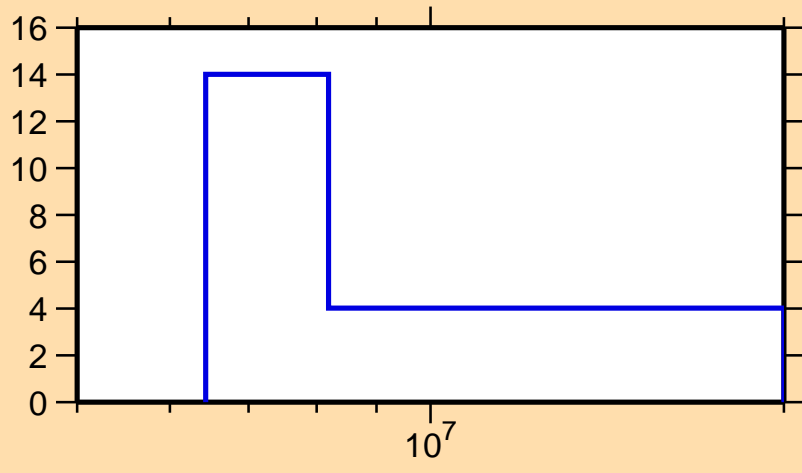
\Delta\sigma/\sigma vs. E for ^{148}\text{Eu}(n,2n)
