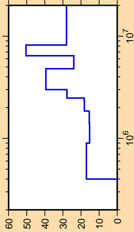
\Delta\sigma/\sigma vs. E for ^{148}\text{Eu}(n,n_4)
