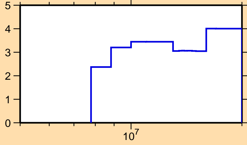
\Delta\sigma/\sigma vs. E for ^{149}\text{Eu}(n,\text{el.})
