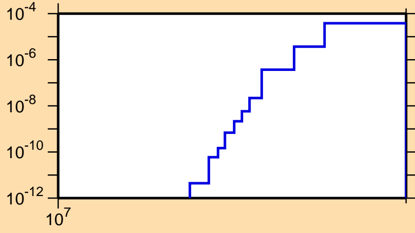
\sigma vs. E for ^{149}\text{Eu}(n,nd)
