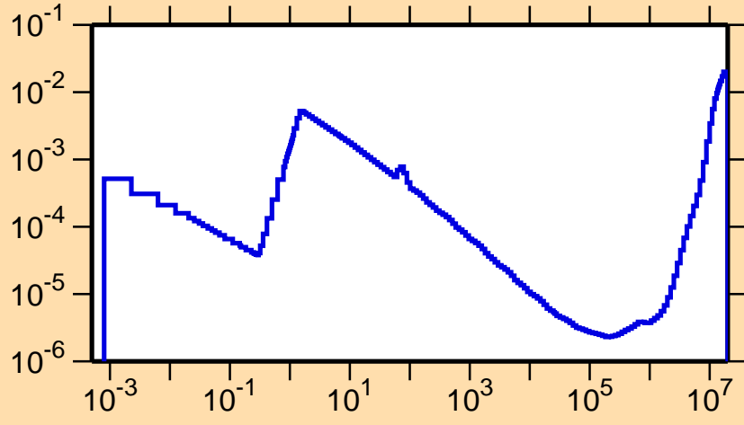
\sigma vs. E for ^{149}\text{Eu}(n,\alpha)
