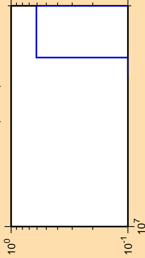
\Delta\sigma/\sigma vs. E for ^{149}\text{Eu} (mt 34)
