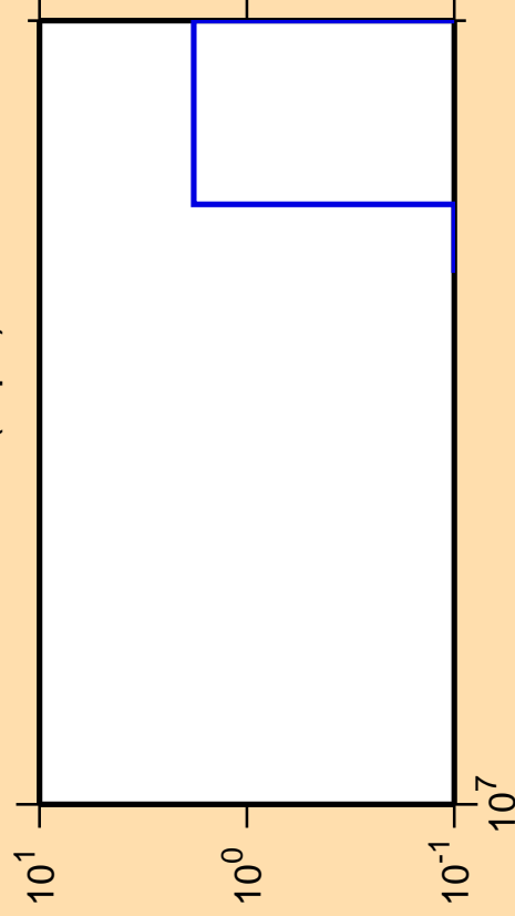
\Delta\sigma/\sigma vs. E for ^{149}\text{Eu}(n,\text{pd})
