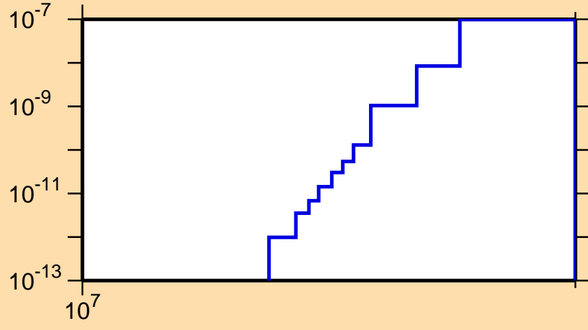
\sigma vs. E for ^{149}\text{Eu}(n,\text{He3})
