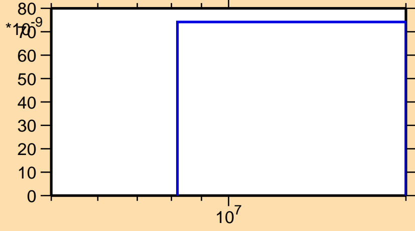
\sigma vs. E for ^{149}\text{Eu}(n,nt)
