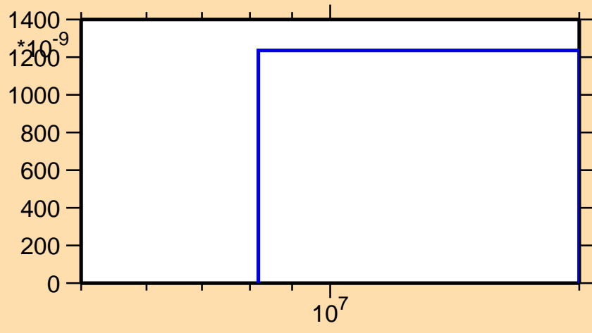
\sigma vs. E for ^{149}\text{Eu}(n,2n\alpha)
