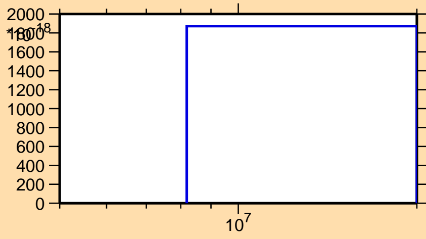
\sigma vs. E for ^{149}\text{Eu}(n,pd)
