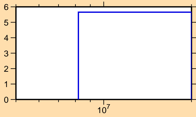
\Delta\sigma/\sigma vs. E for ^{149}\text{Eu}(n,\text{inel.})
