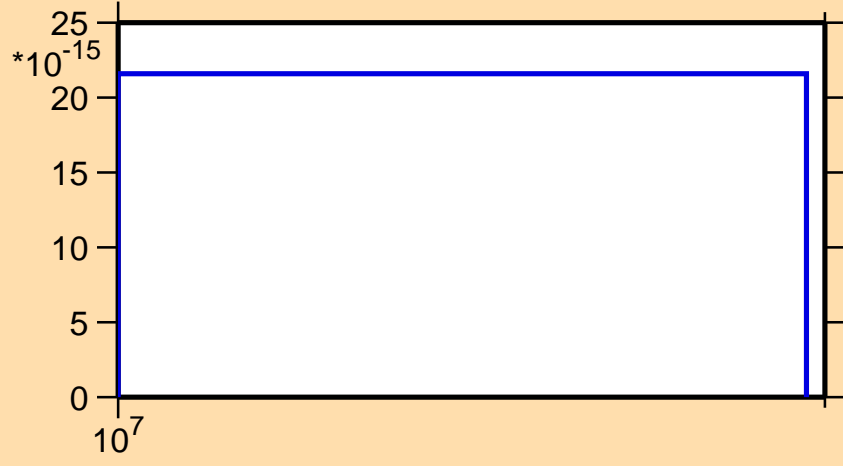
\sigma vs. E for ^{150}\text{Eu} (mt 34)
