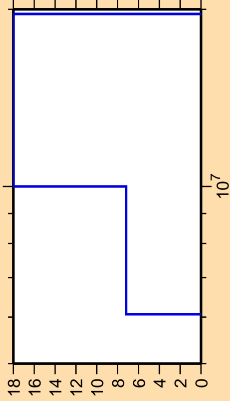
\Delta\sigma/\sigma vs. E for ^{150}\text{Eu}(n,n\text{cont.})
