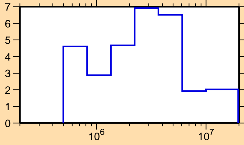
\Delta\sigma/\sigma vs. E for ^{150}\text{Eu}(n, \text{el.})
