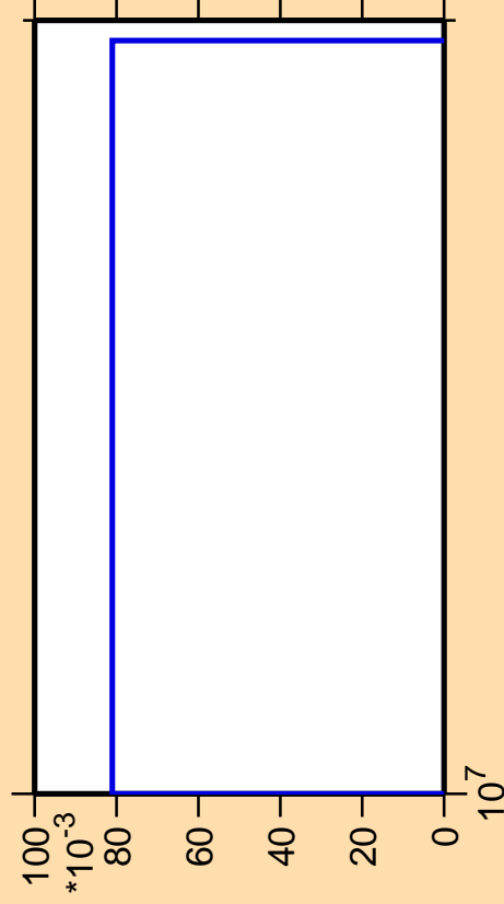
\Delta\sigma/\sigma vs. E for ^{150}\text{Eu} (mt 34)
