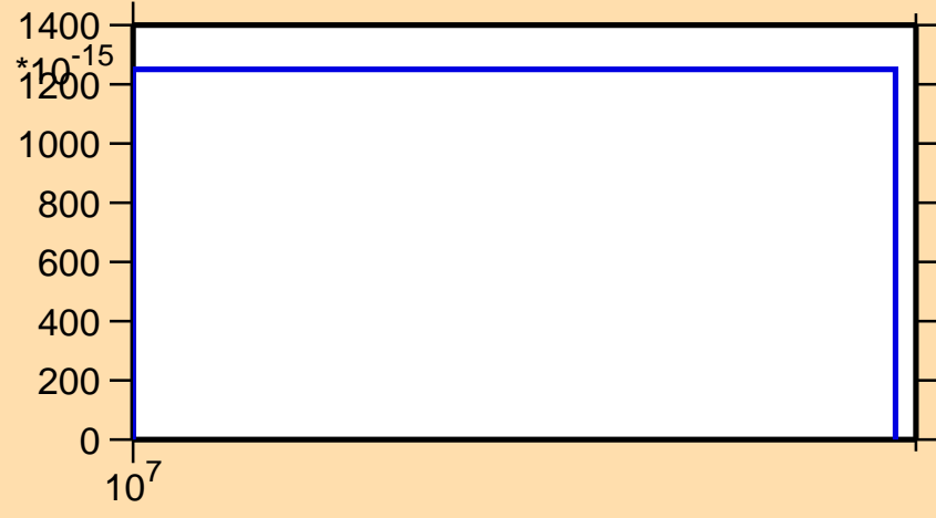
\sigma vs. E for ^{150}\text{Eu} (mt 45)
