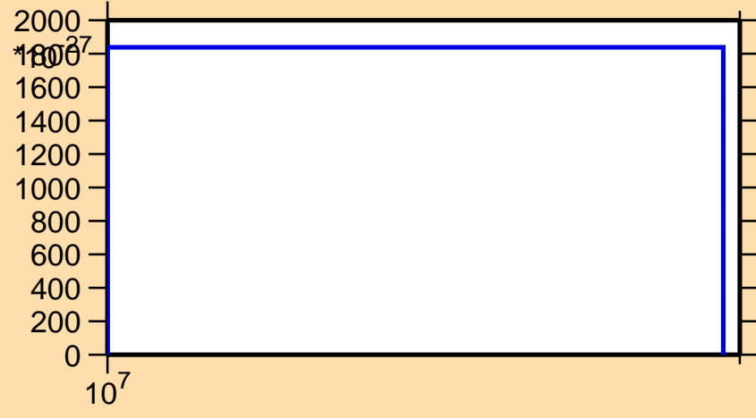
\sigma vs. E for ^{150}\text{Eu} (mt 42)
