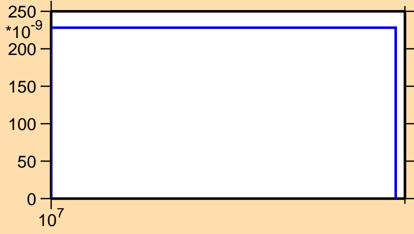
\sigma vs. E for ^{150}\text{Eu}(n,nt)
