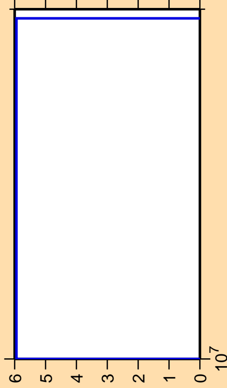
\Delta\sigma/\sigma vs. E for ^{150}\text{Eu}(\text{mt117})
