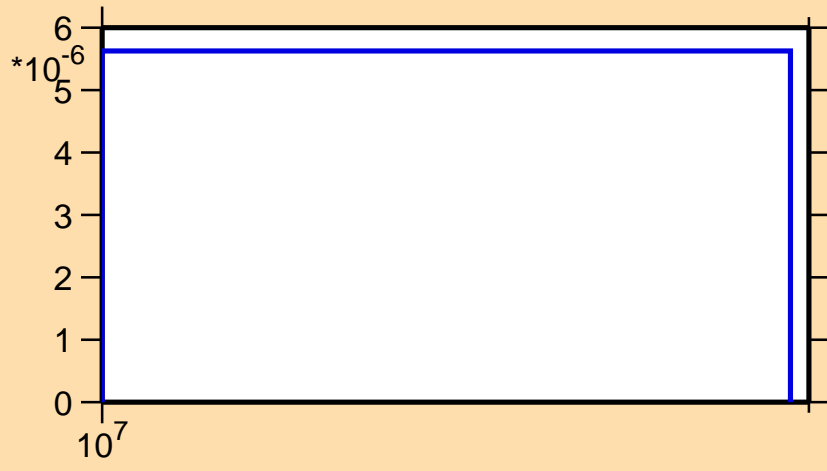
\sigma vs. E for ^{150}\text{Eu}(n,2np)
