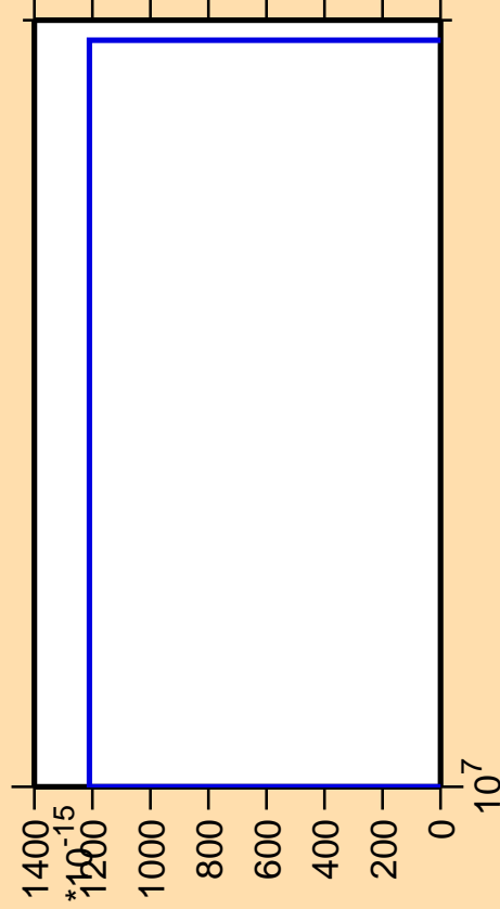
\Delta\sigma/\sigma vs. E for ^{150}\text{Eu} (mt 42)
