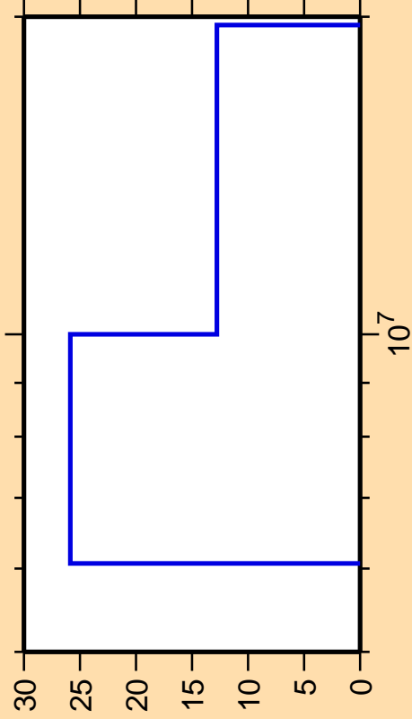
\Delta\sigma/\sigma vs. E for ^{150}\text{Eu}(n,n_1)
