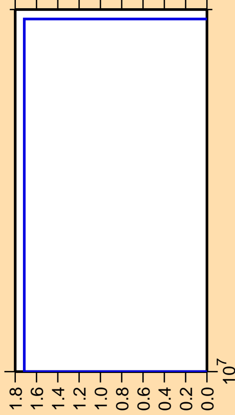
\Delta\sigma/\sigma vs. E for ^{150}\text{Eu} (mt 45)
