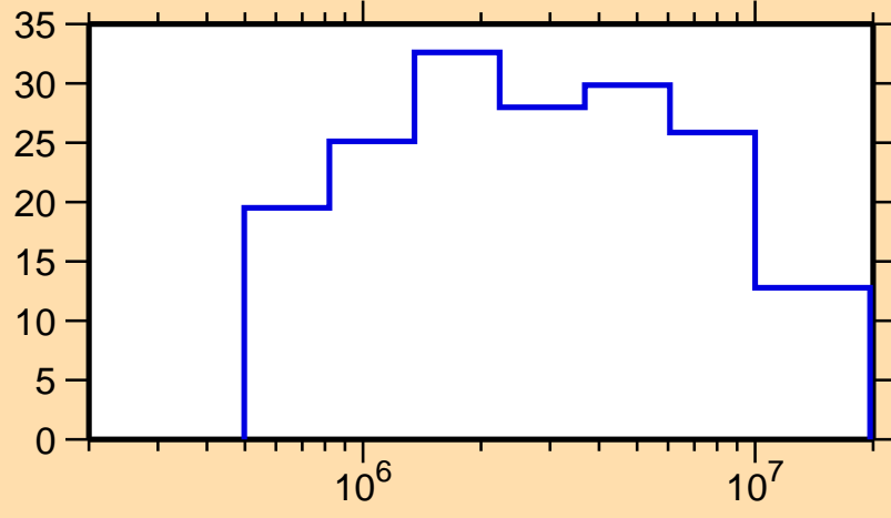
\Delta\sigma/\sigma vs. E for ^{150}\text{Eu}(n, n_1)
