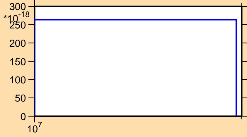
\sigma vs. E for ^{150}\text{Eu}(n,pt)
