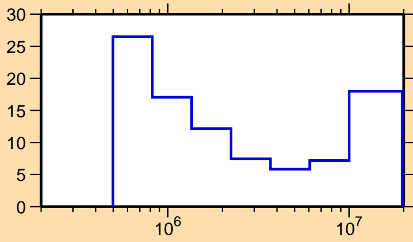
\Delta\sigma/\sigma vs. E for ^{150}\text{Eu}(n,n\text{cont.})
