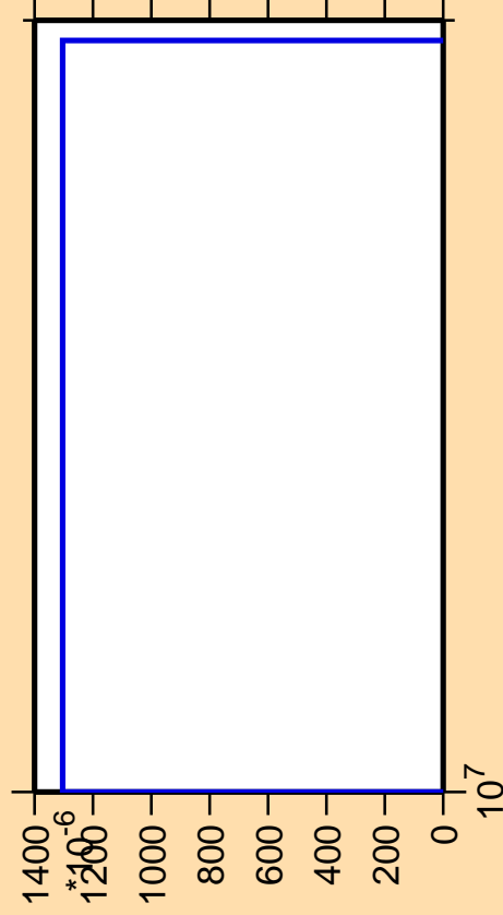
\Delta\sigma/\sigma vs. E for ^{150}\text{Eu}(n,pt)
