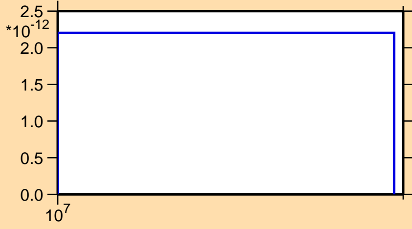
\sigma vs. E for ^{150}\text{Eu}(\text{mt117})
