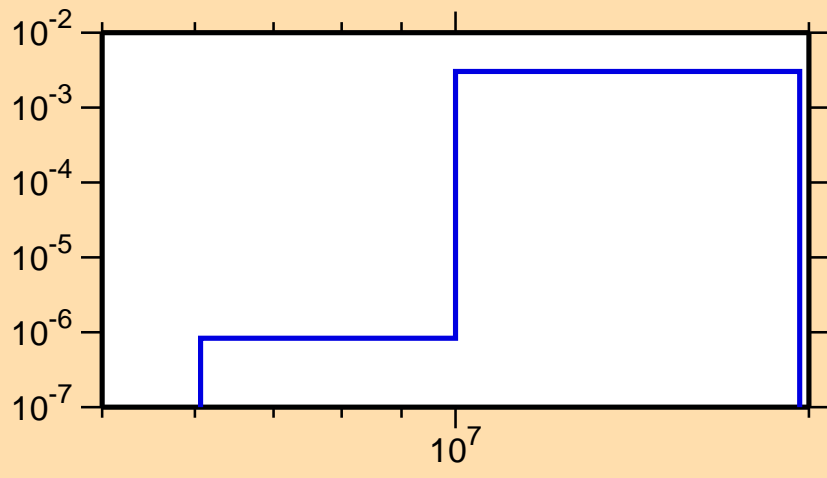
\sigma vs. E for ^{150}\text{Eu}(n,np)
