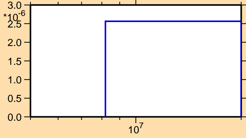
\sigma vs. E for ^{150}\text{Eu}(n,nd)
