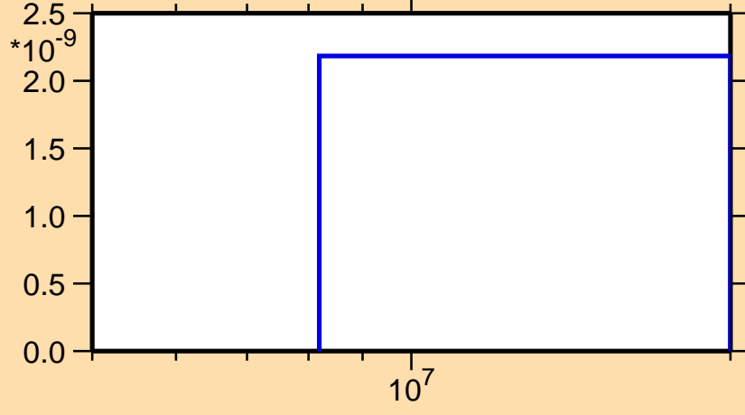
\sigma vs. E for ^{150}\text{Eu}(n,p\alpha)
