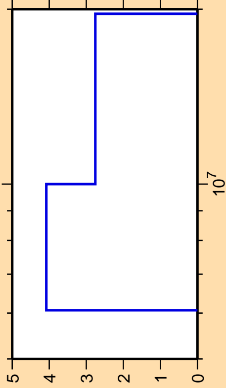
\Delta\sigma/\sigma vs. E for ^{150}\text{Eu}(n,2n)
