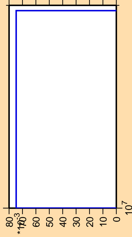
\Delta\sigma/\sigma vs. E for ^{150}\text{Eu}(n,3n\alpha)
