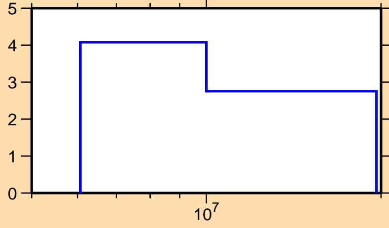
\Delta\sigma/\sigma vs. E for ^{150}\text{Eu}(n,2n)
