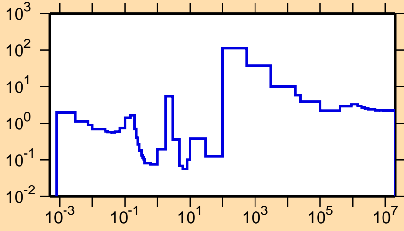
\sigma vs. E for ^{150}\text{Eu}(n,\text{nonel.})
