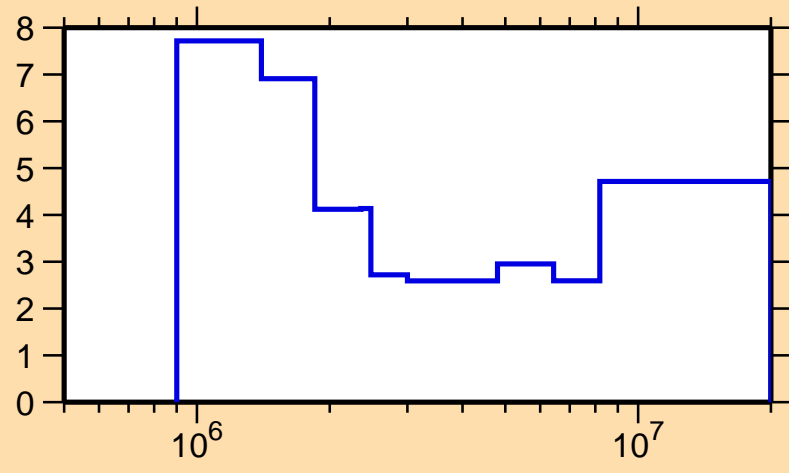
\Delta\sigma/\sigma vs. E for ^{151}\text{Eu}(n,n\text{cont.})
