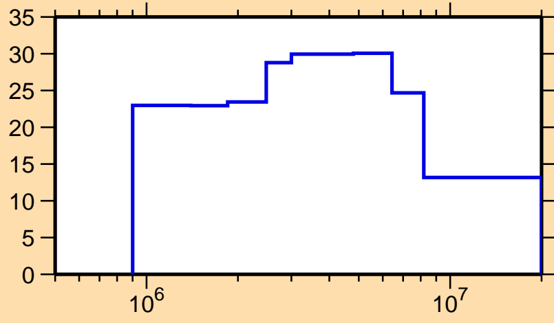
\Delta\sigma/\sigma vs. E for ^{151}\text{Eu}(n,p)
