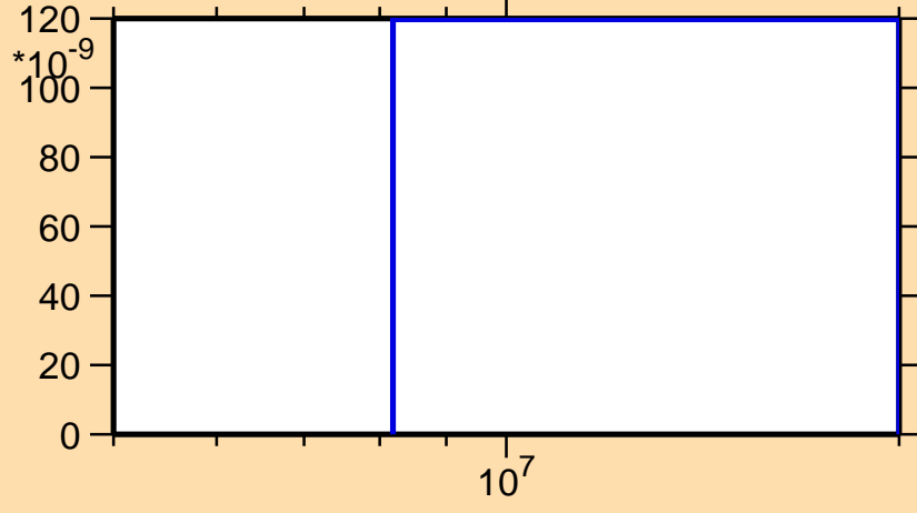
\sigma vs. E for ^{151}\text{Eu}(n,2n\alpha)
