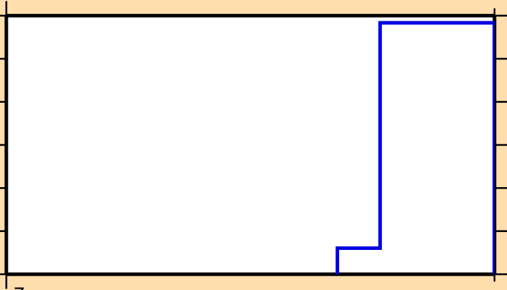
\sigma vs. E for ^{152}\text{Eu}(\text{mt117})
