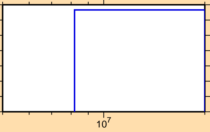
\sigma vs. E for ^{152}\text{Eu}(n,nt)
