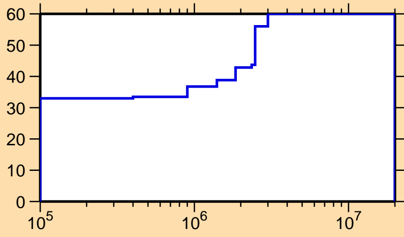
\Delta\sigma/\sigma vs. E for ^{152}\text{Eu}(n, n_1)
