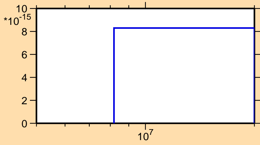
\sigma vs. E for ^{152}\text{Eu}(\text{mt117})
