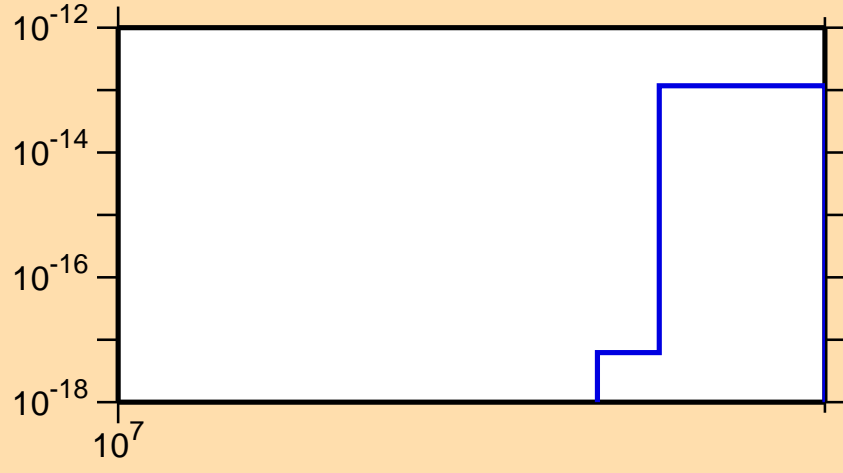
\sigma vs. E for ^{152}\text{Eu} (mt 34)
