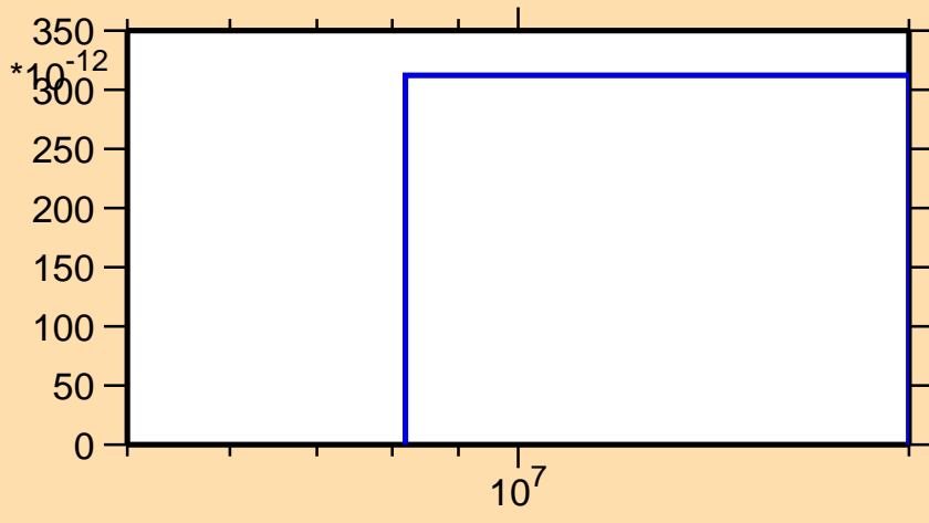
\sigma vs. E for ^{152}\text{Eu}(n,\text{He3})
