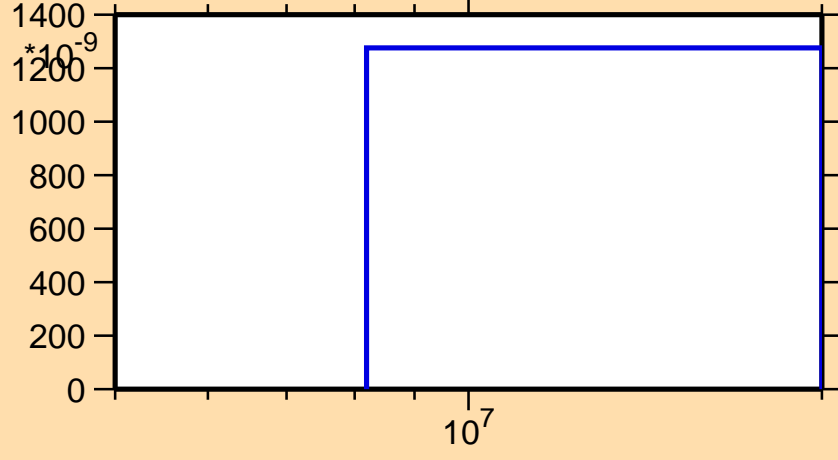
\sigma vs. E for ^{152}\text{Eu}(n,nd)
