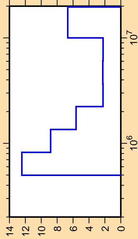
\Delta\sigma/\sigma vs. E for ^{153}\text{Eu}(n,\text{ncont.})
