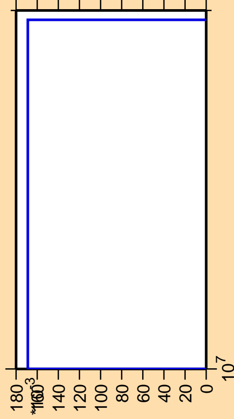
\Delta\sigma/\sigma vs. E for ^{153}\text{Eu}(n,p\alpha)
