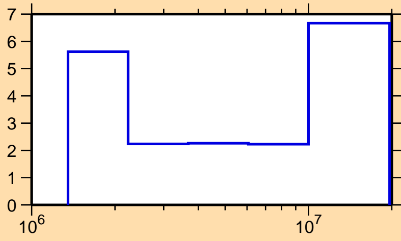
\Delta\sigma/\sigma vs. E for ^{153}\text{Eu}(n,n\text{cont.})
