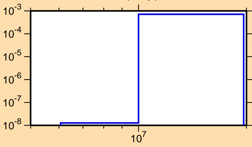
\sigma vs. E for ^{153}\text{Eu}(n,np)
