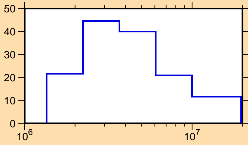
\Delta\sigma/\sigma vs. E for ^{153}\text{Eu}(n,p)
