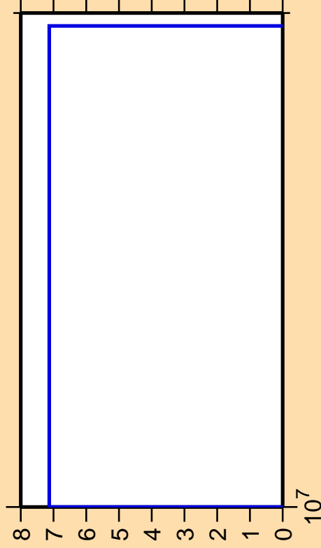
\Delta\sigma/\sigma vs. E for ^{153}\text{Eu}(n,3n)
