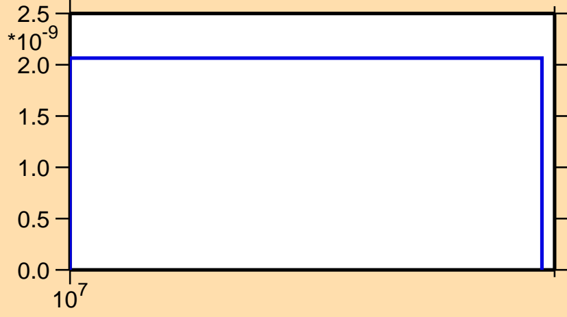
\sigma vs. E for ^{153}\text{Eu}(n,2n\alpha)
