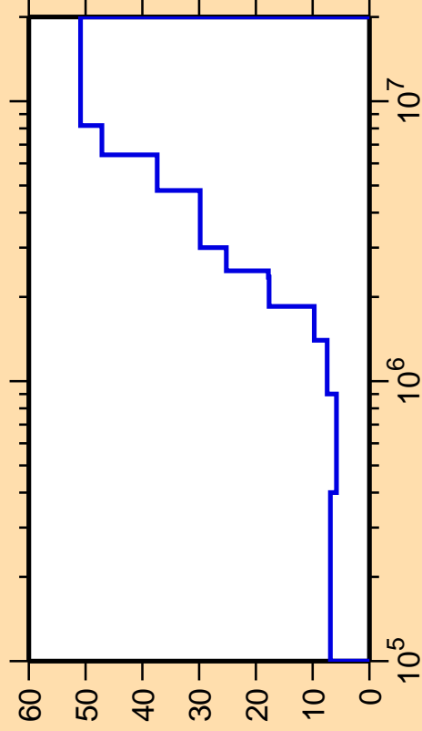
\Delta\sigma/\sigma vs. E for ^{153}\text{Eu}(n,n_4)
