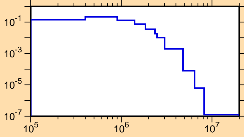
\sigma vs. E for ^{153}\text{Eu}(n,n_4)
