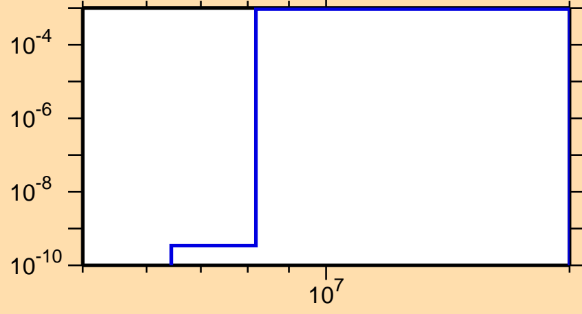
\sigma vs. E for ^{153}\text{Eu}(n,d)
