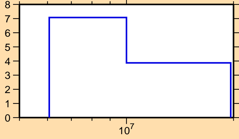
\Delta\sigma/\sigma vs. E for ^{154}\text{Eu}(n,2n)
