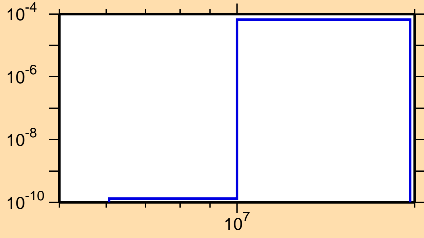
\sigma vs. E for ^{154}\text{Eu}(n,n\alpha)
