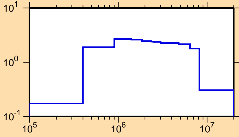
\sigma vs. E for ^{154}\text{Eu}(n,n\text{cont.})
