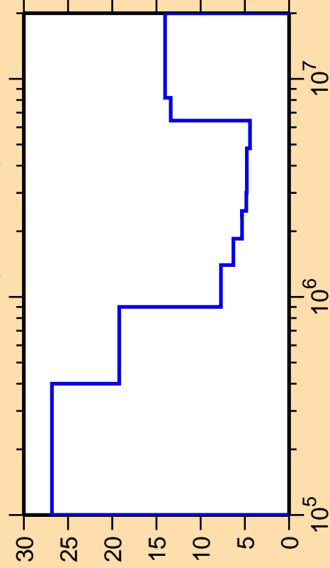
\Delta\sigma/\sigma vs. E for ^{154}\text{Eu}(n,\text{ncont.})
