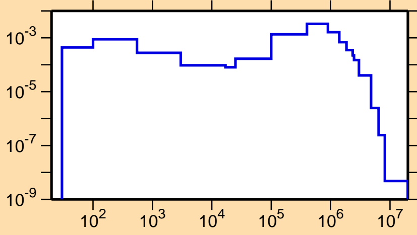
\sigma vs. E for ^{154}\text{Eu}(n,n_1)
