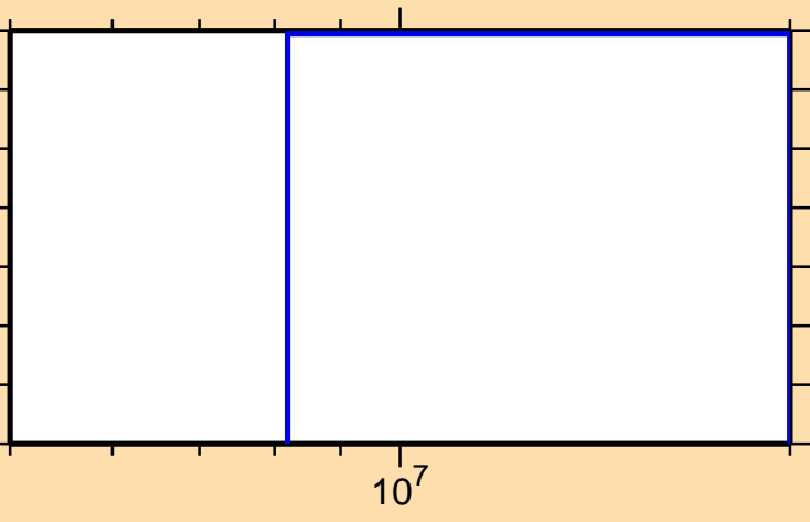
\sigma vs. E for ^{154}\text{Eu}(n,\text{He3})
