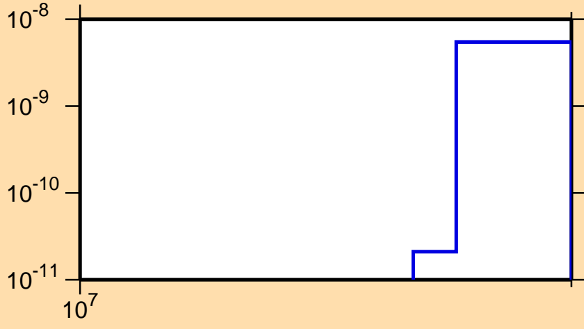
\sigma vs. E for ^{155}\text{Eu}(n,2n\alpha)
