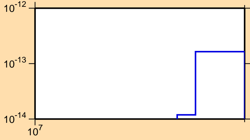
\sigma vs. E for ^{155}\text{Eu}(n,p\alpha)
