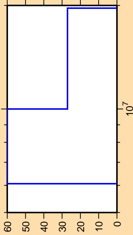
\Delta\sigma/\sigma vs. E for ^{155}\text{Eu}(n,np)
