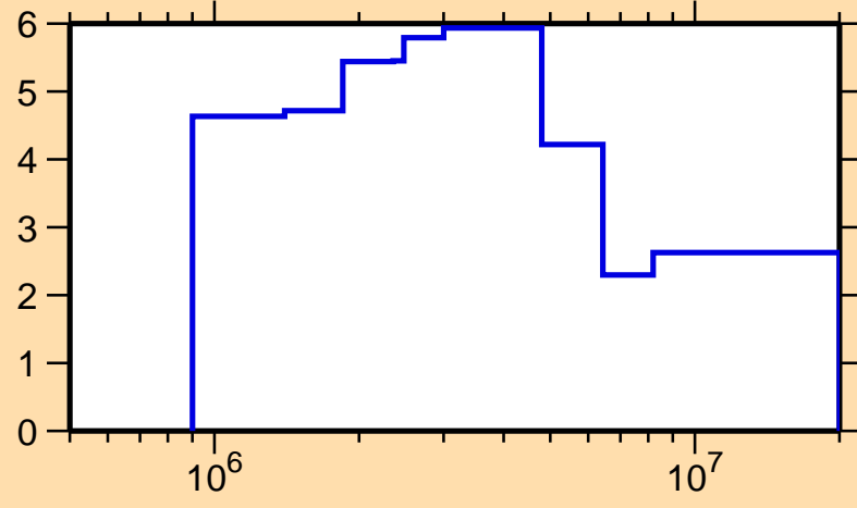
\Delta\sigma/\sigma vs. E for ^{155}\text{Eu}(n, el.)
