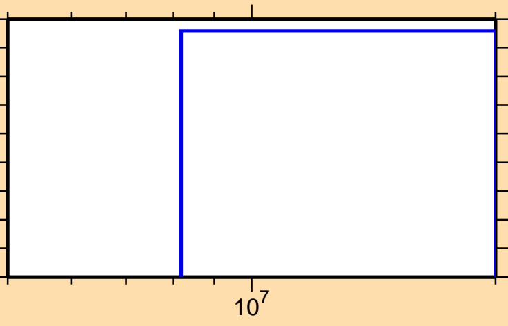
\sigma vs. E for ^{155}\text{Eu}(n,t)
