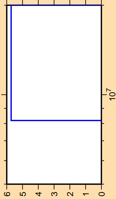
\Delta\sigma/\sigma vs. E for ^{155}\text{Eu}(n,3n)
