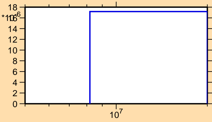
\sigma vs. E for ^{155}\text{Eu}(n,t)
