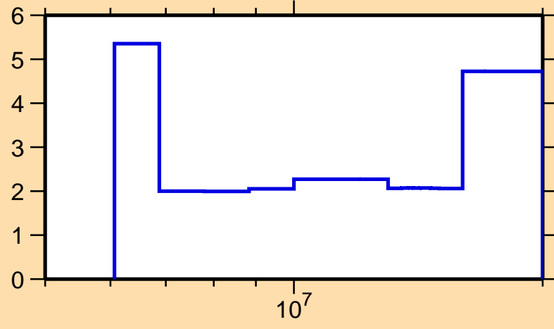
\Delta\sigma/\sigma vs. E for ^{156}\text{Eu}(n,\text{el.})
