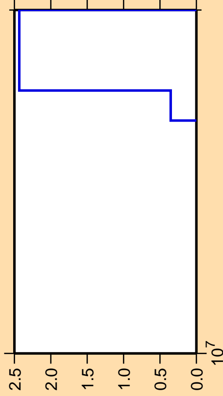
\Delta\sigma/\sigma vs. E for ^{156}\text{Eu}(n,p\alpha)
