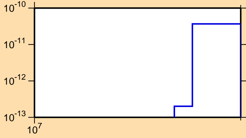
\sigma vs. E for ^{156}\text{Eu}(n,\text{He3})
