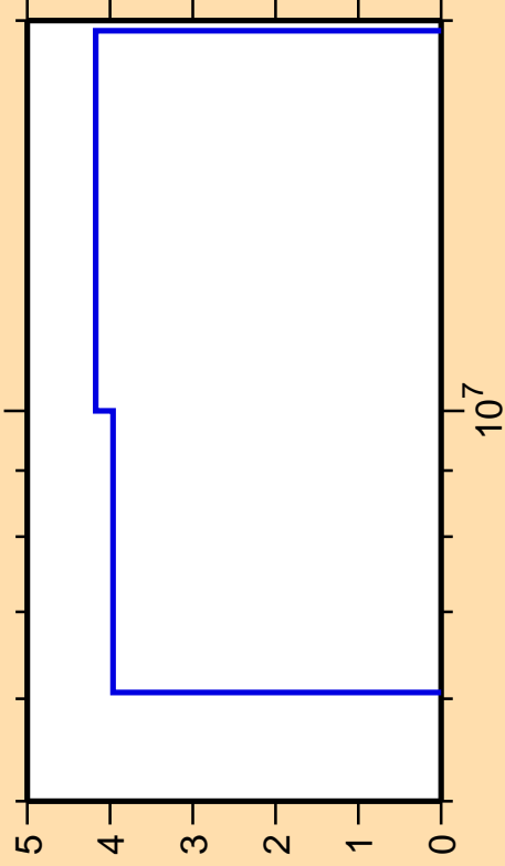
\Delta\sigma/\sigma vs. E for ^{156}\text{Eu}(n,2n)
