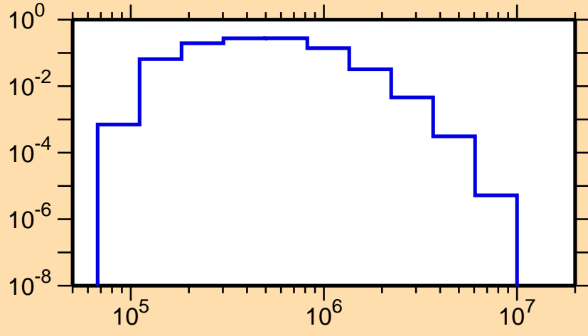
\sigma vs. E for ^{156}\text{Eu}(n,n_4)
