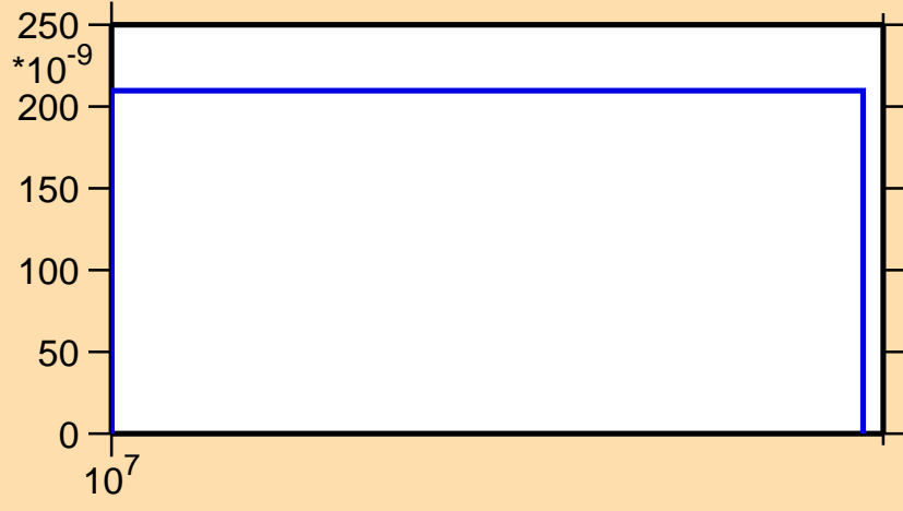
\sigma vs. E for ^{156}\text{Eu}(n,\text{nd})
