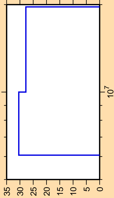
\Delta\sigma/\sigma vs. E for ^{156}\text{Eu}(n,p)
