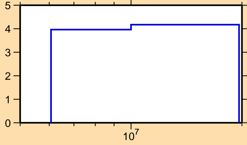
\Delta\sigma/\sigma vs. E for ^{156}\text{Eu}(n,2n)
