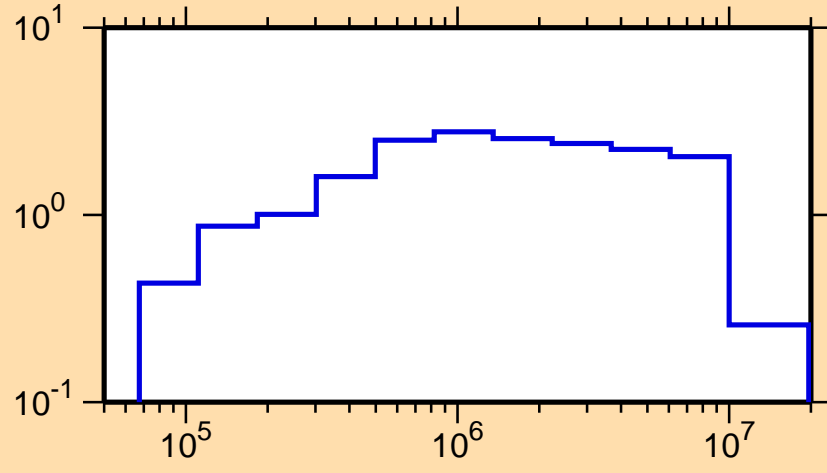
\sigma vs. E for ^{157}\text{Eu}(n,\text{inel.})
