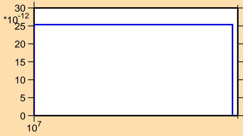
\sigma vs. E for ^{157}\text{Eu}(n,2n\alpha)
