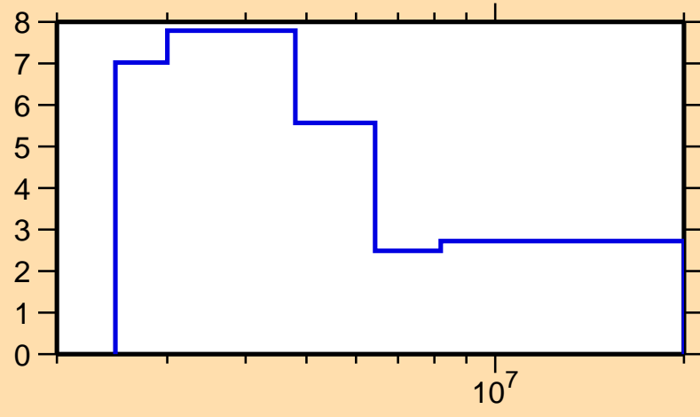
\Delta\sigma/\sigma vs. E for ^{157}\text{Eu}(n,\text{el.})
