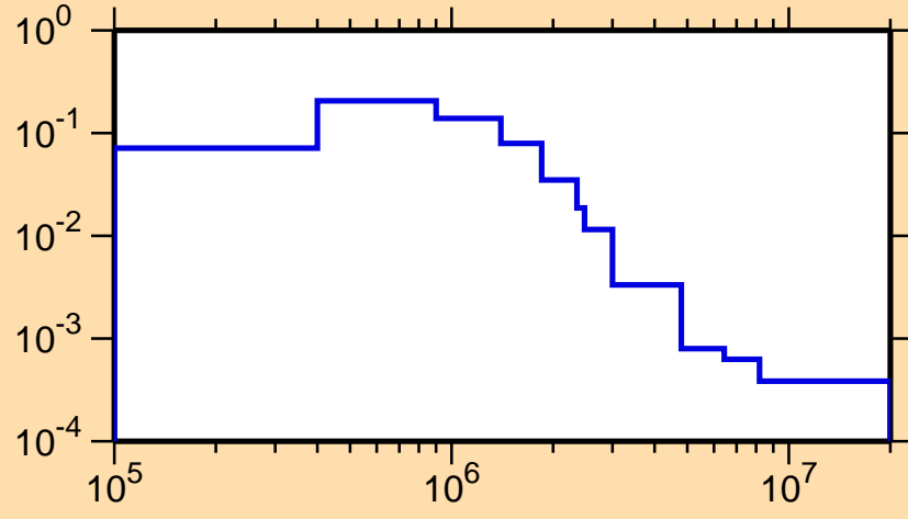
\sigma vs. E for ^{157}\text{Eu}(n,n_3)
