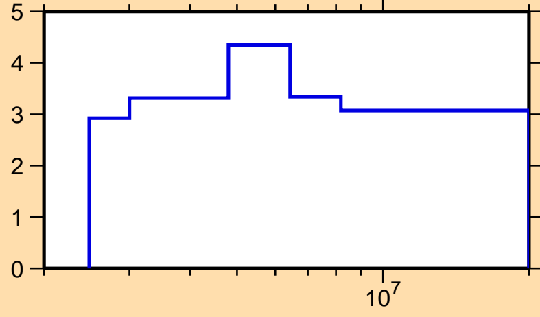
\Delta\sigma/\sigma vs. E for ^{157}\text{Eu}(n,\text{nonel.})
