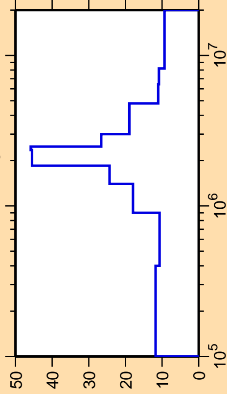
\Delta\sigma/\sigma vs. E for ^{157}\text{Eu}(n,n_3)
