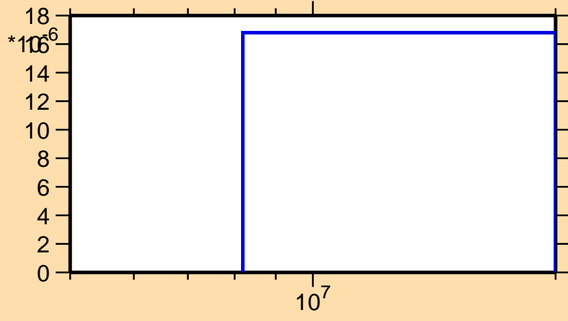
\sigma vs. E for ^{157}\text{Eu}(n,t)
