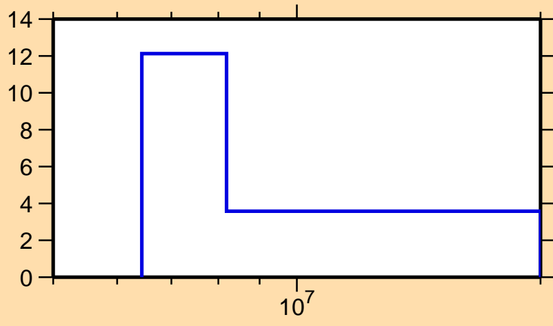
\Delta\sigma/\sigma vs. E for ^{157}\text{Eu}(n,2n)
