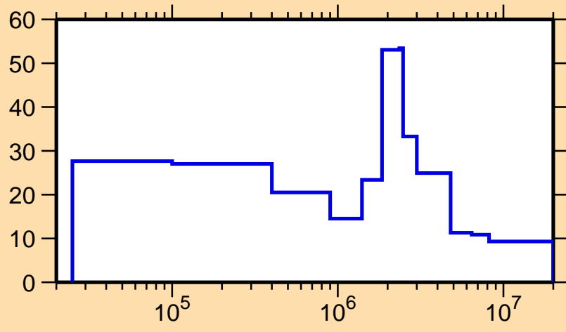
\Delta\sigma/\sigma vs. E for ^{157}\text{Eu}(n,n_1)
