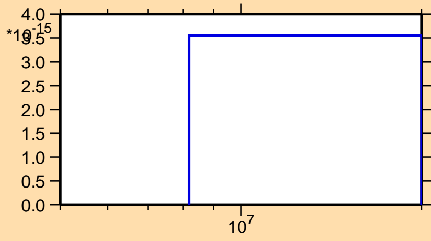
\sigma vs. E for ^{157}\text{Eu}(n,\text{He3})
