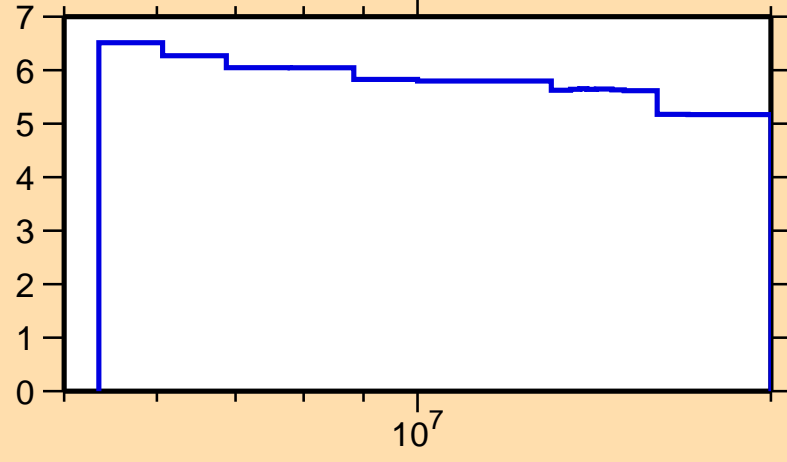
\Delta\sigma/\sigma vs. E for ^{158}\text{Eu}(n,\text{nonel.})
