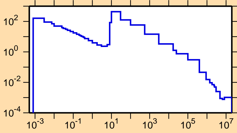
\sigma vs. E for ^{158}\text{Eu}(n,\gamma)
