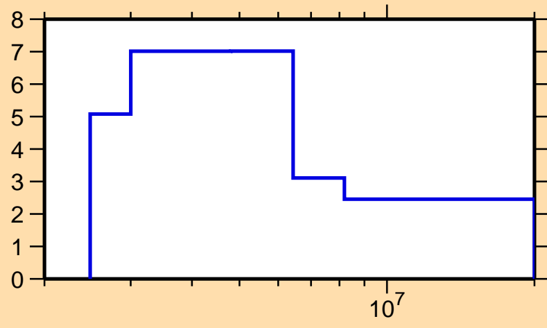
\Delta\sigma/\sigma vs. E for ^{158}\text{Eu}(n,\text{tot.})
