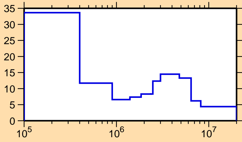
\Delta\sigma/\sigma vs. E for ^{158}\text{Eu}(n, el.)
