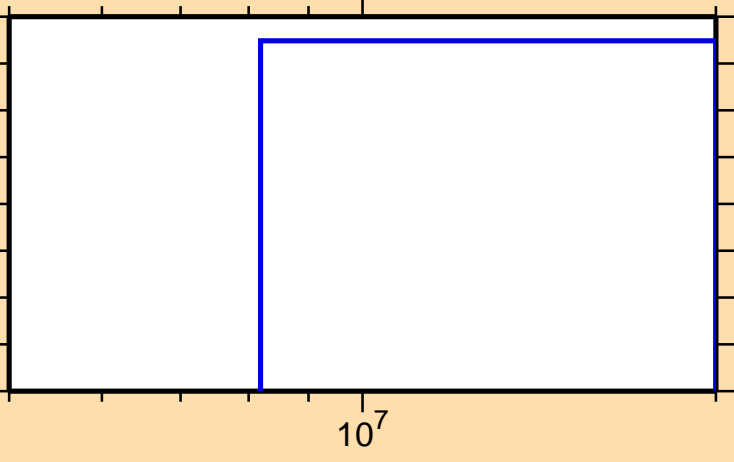
\sigma vs. E for ^{158}\text{Eu}(n,\text{He3})
