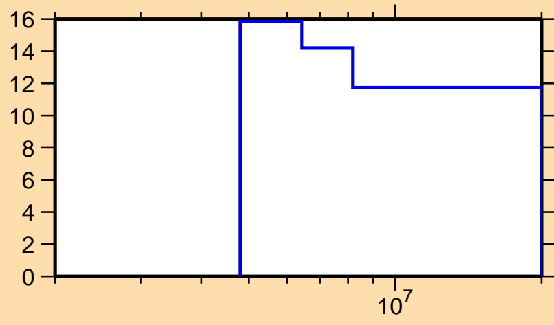
\Delta\sigma/\sigma vs. E for ^{158}\text{Eu}(n,2n)
