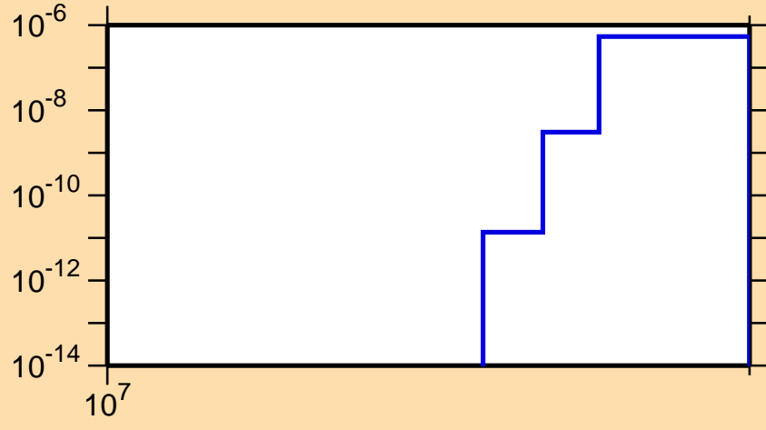
\sigma vs. E for ^{159}\text{Eu}(n,nd)
