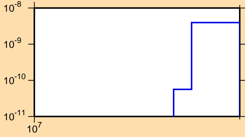
\sigma vs. E for ^{159}\text{Eu}(n,2n\alpha)
