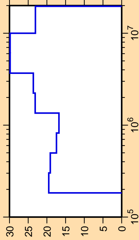
\Delta\sigma/\sigma vs. E for ^{159}\text{Eu}(n,n_4)
