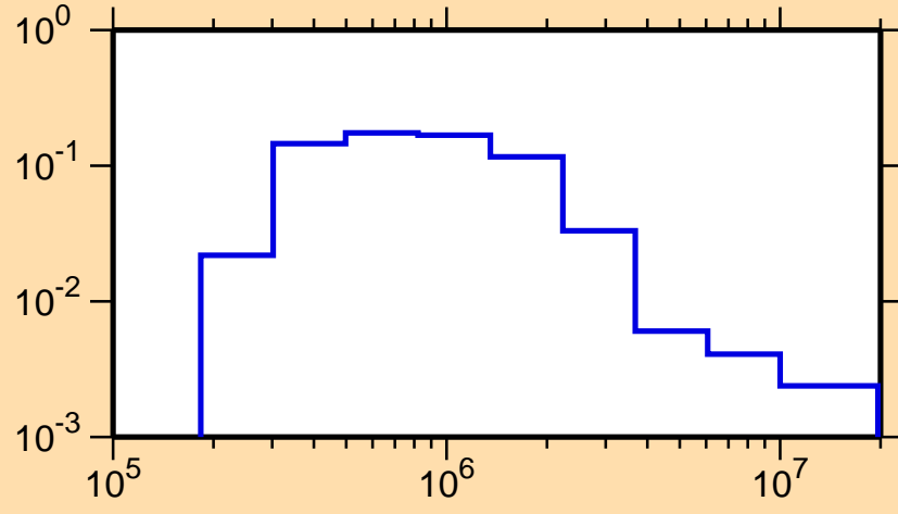
\sigma vs. E for ^{159}\text{Eu}(n,n_4)
