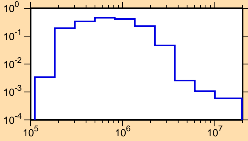
\sigma vs. E for ^{159}\text{Eu}(n,n_2)
