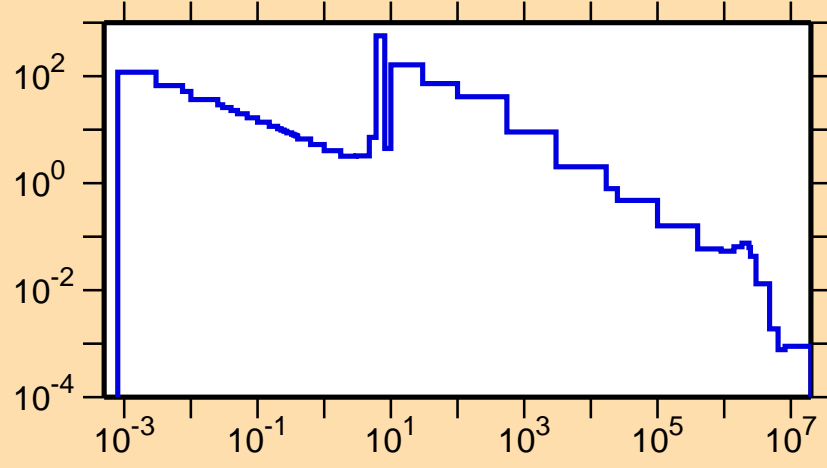
\sigma vs. E for ^{159}\text{Eu}(n,\gamma)
