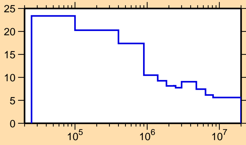
\Delta\sigma/\sigma vs. E for ^{159}\text{Eu}(n,\text{nonel.})
