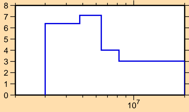
\Delta\sigma/\sigma vs. E for ^{159}\text{Eu}(n,\text{tot.})
