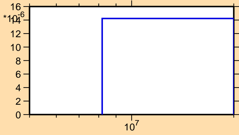
\sigma vs. E for ^{159}\text{Eu}(n,t)
