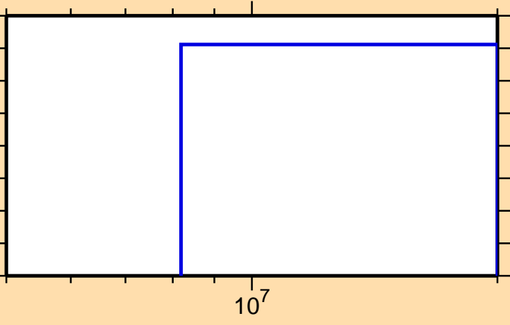
\sigma vs. E for ^{159}\text{Eu}(n,t)
