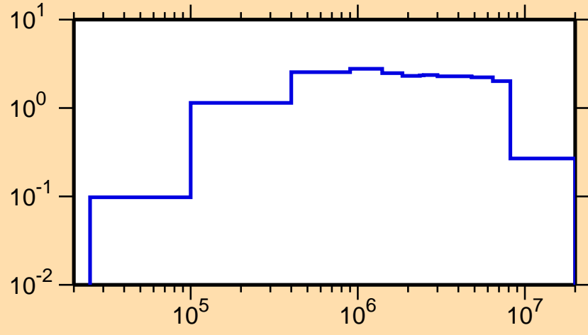
\sigma vs. E for ^{159}\text{Eu}(n,\text{inel.})
