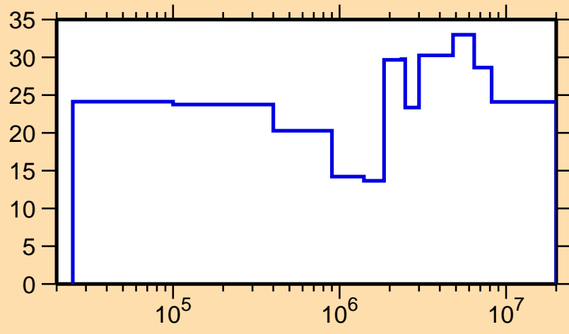
\Delta\sigma/\sigma vs. E for ^{159}\text{Eu}(n,n_1)
