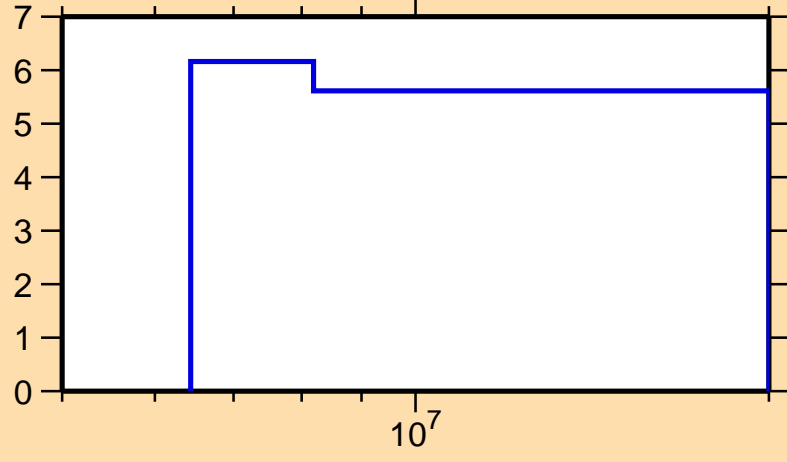
\Delta\sigma/\sigma vs. E for ^{159}\text{Eu}(n,\text{nonel.})
