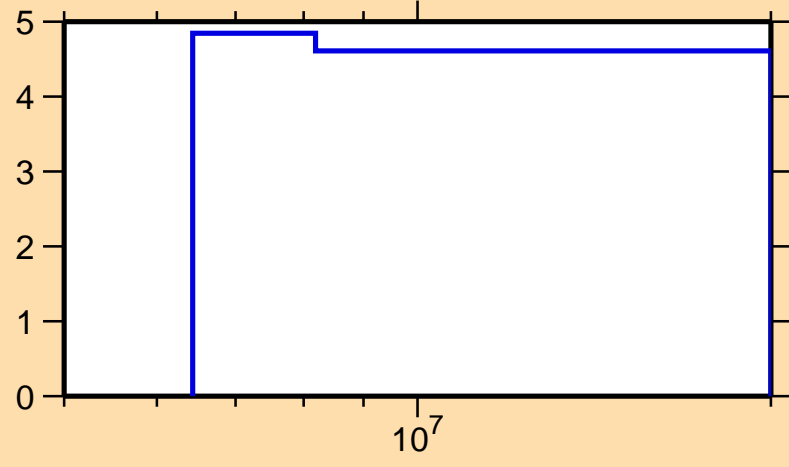
\Delta\sigma/\sigma vs. E for ^{159}\text{Eu}(n,\text{el.})
