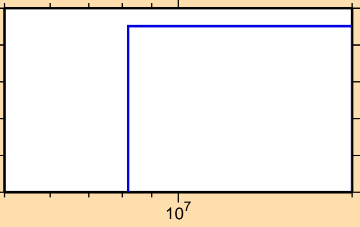
\sigma vs. E for ^{159}\text{Eu}(n,nd)
